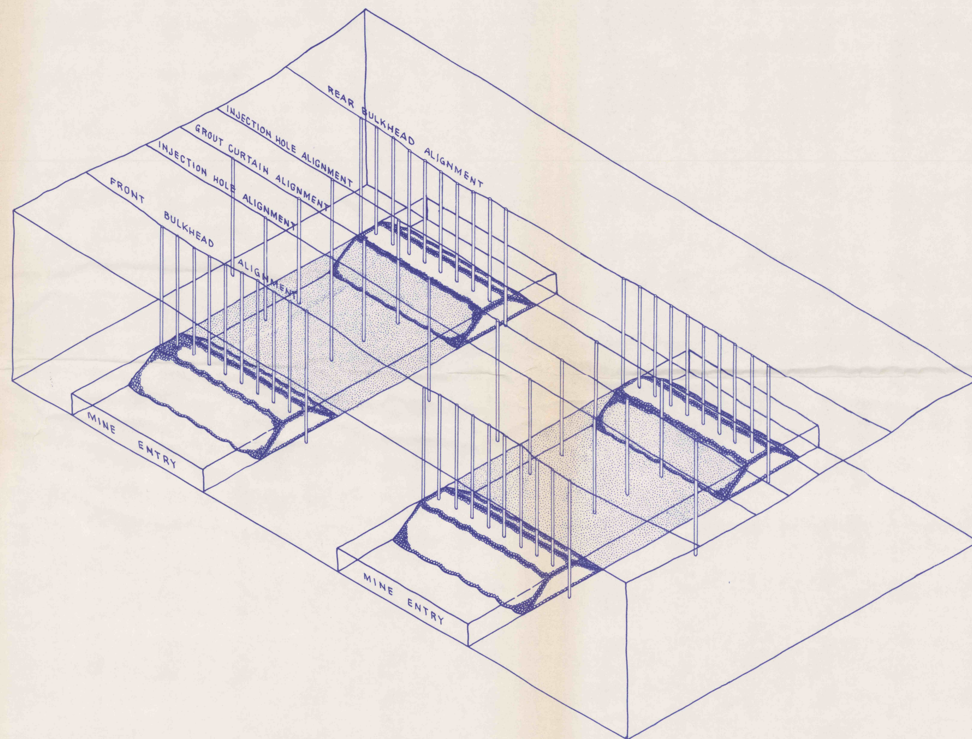
ISOMETRIC DRAWING OF DOUBLE BULKHEAD DEEP MINE SEAL NO SCALE
