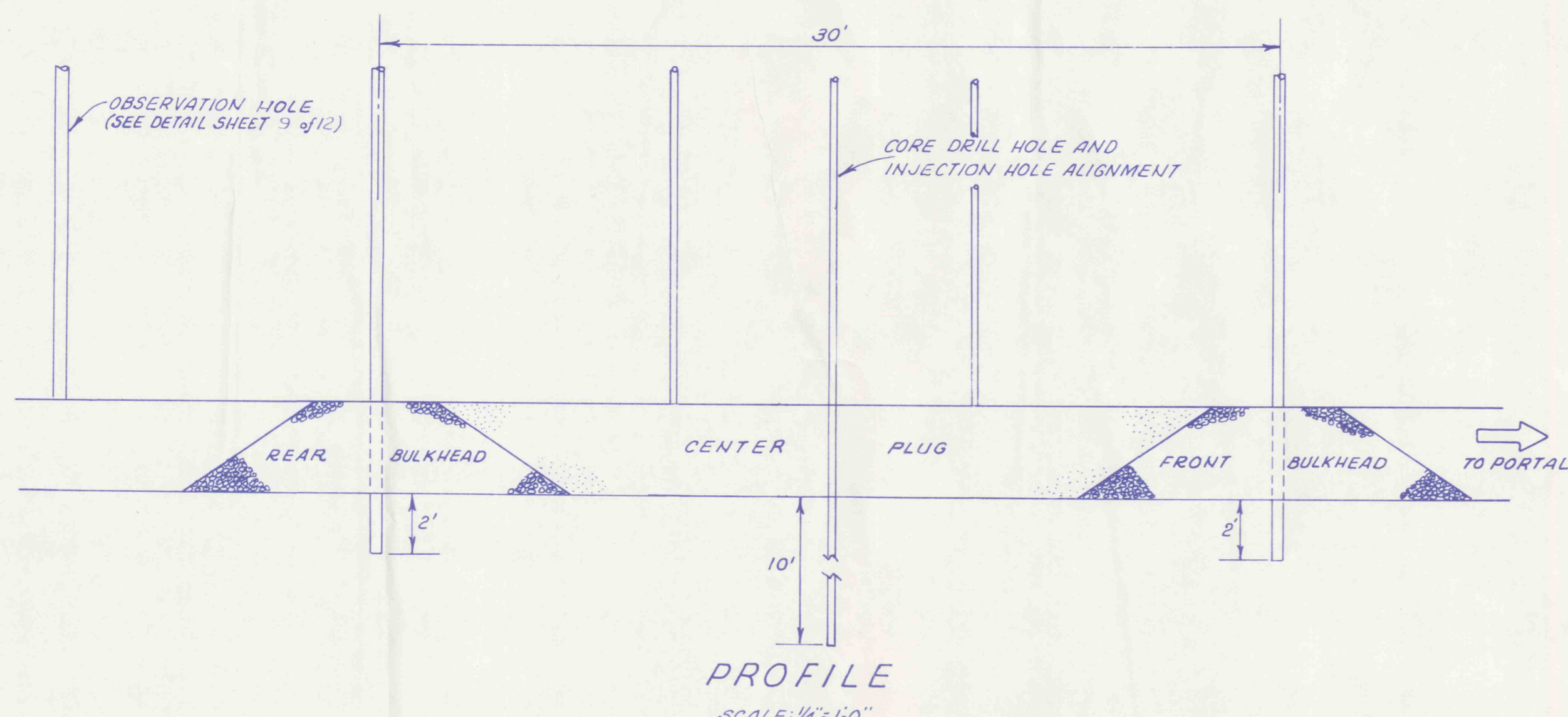
CONSTRUCTION DRAWING OF DEEP MINE SEAL
