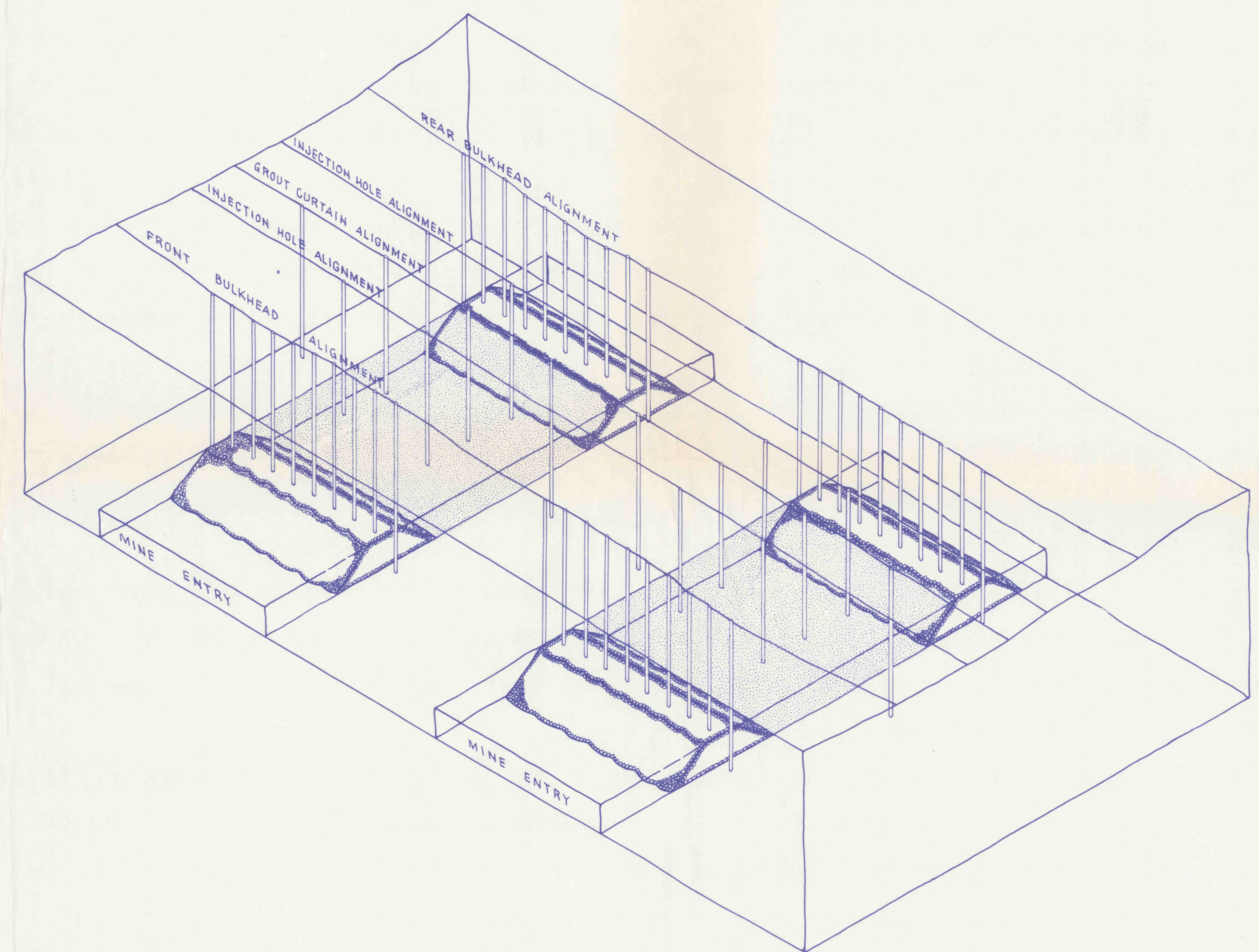
ISOMETRIC DRAWING OF DOUBLE BULKHEAD DEEP MINE SEAL NO SCALE
