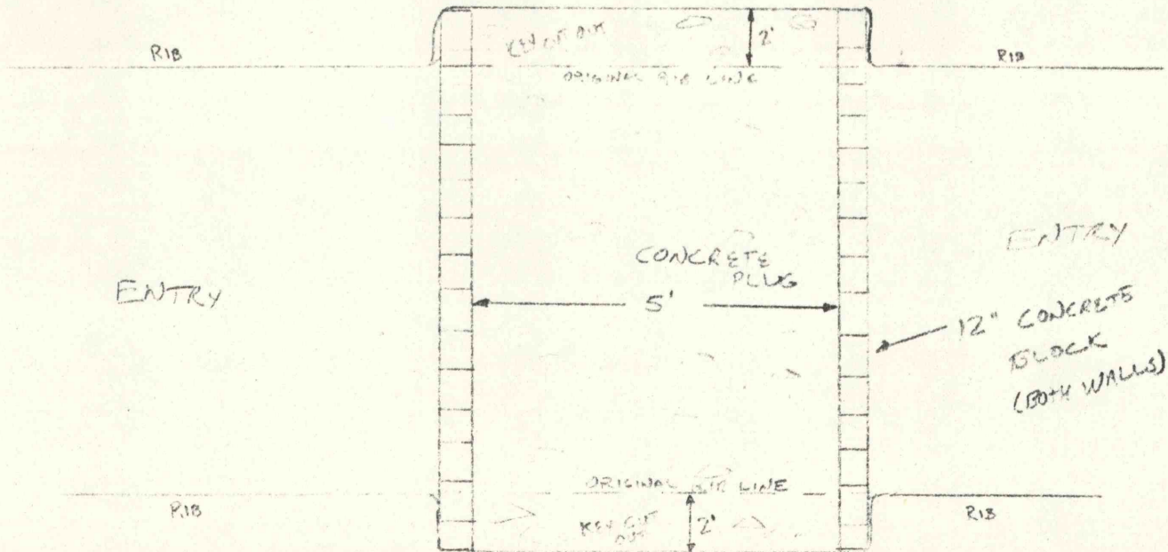
TOP VIEW
