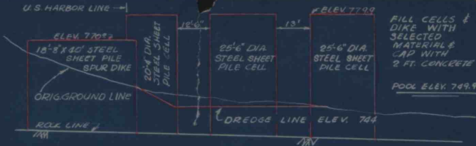
SECTION AT SPUR DIKE & ICEBREAKER
