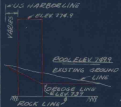
TYPICAL SECTION - MOORING PIER & ICEBREAKER
