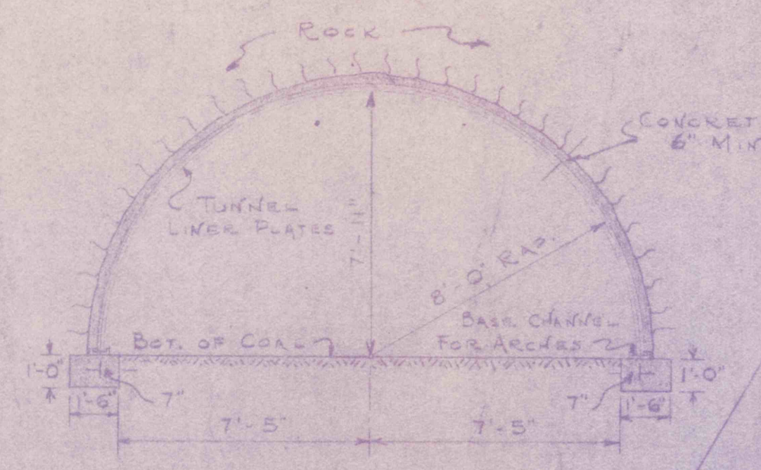
SECTION "B-B" SCALE 1/4" = 1'-0"
