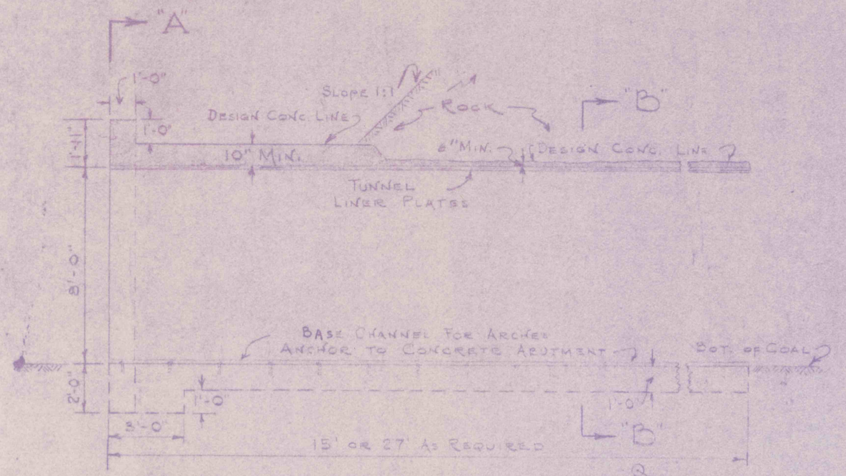
TYPICAL LONGITUDINAL SECTION SCALE 1/4" = 1'-0"
