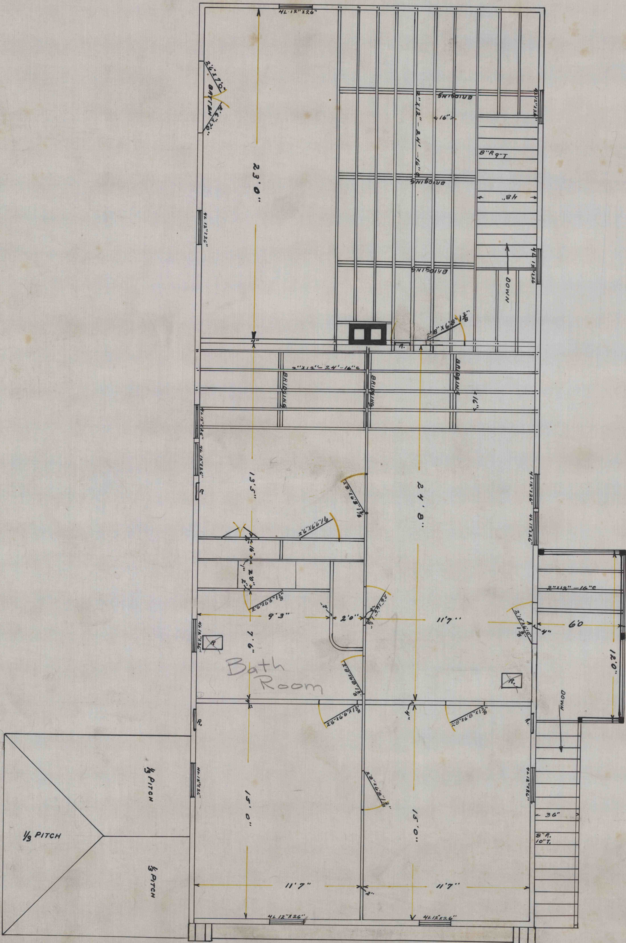
SECOND FLOOR PLAN SCALE \frac{1}{4}'' = 1'
