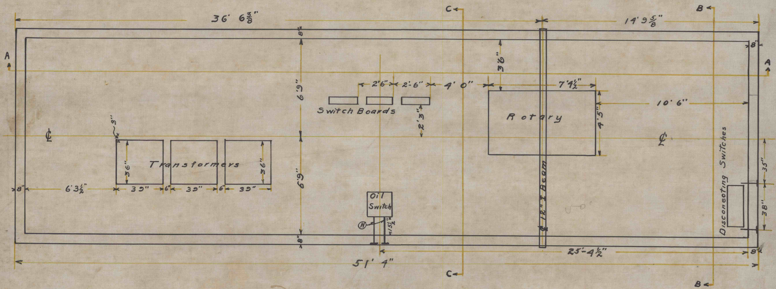
FLOOR PLAN Scale 1/4" = 1'
