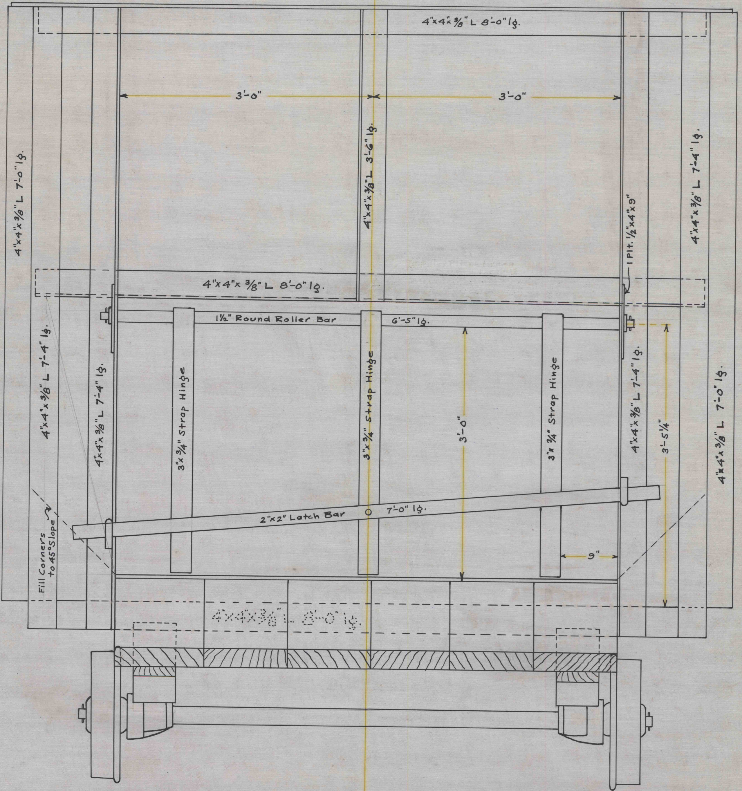
FRONT ELEVATION
