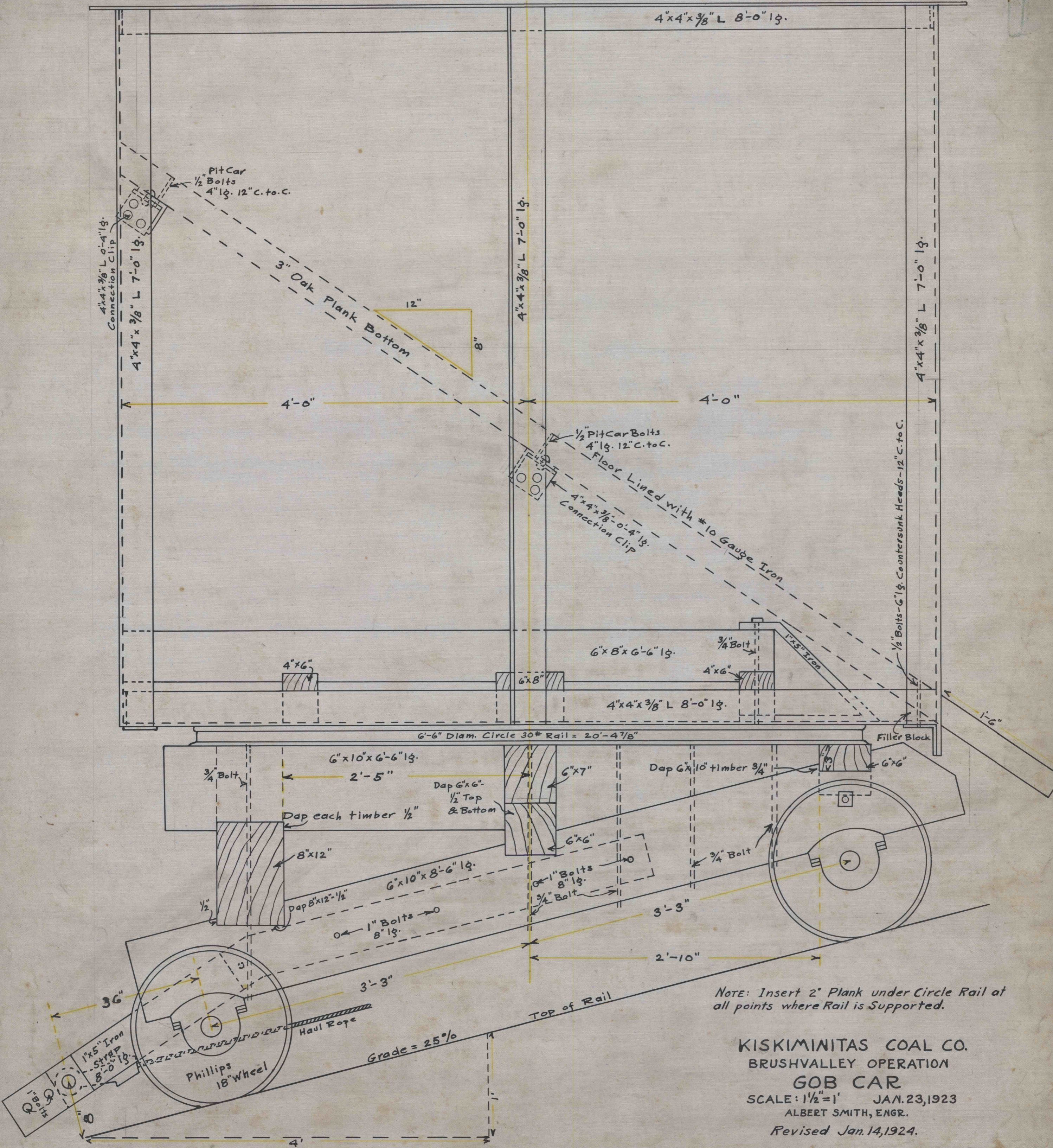
SIDE ELEVATION
