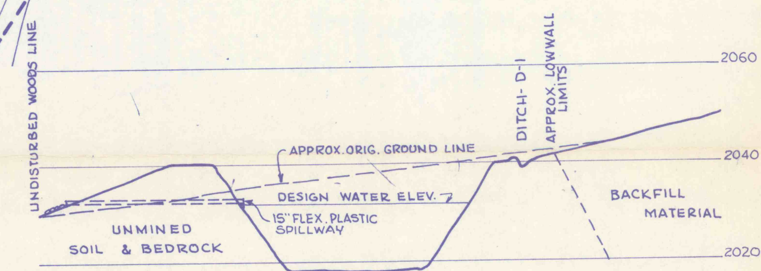
SECTION A-A' SCALE: 1"=40' HOR. 1"=20' VER.
