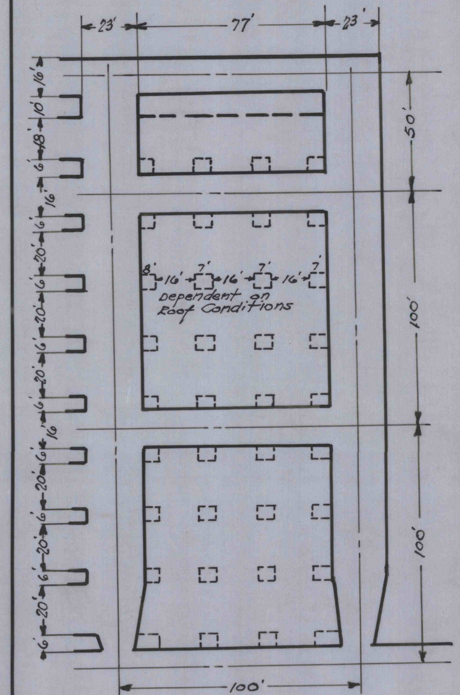
DETAIL OF ROOM PILLARING 1" = 40'
