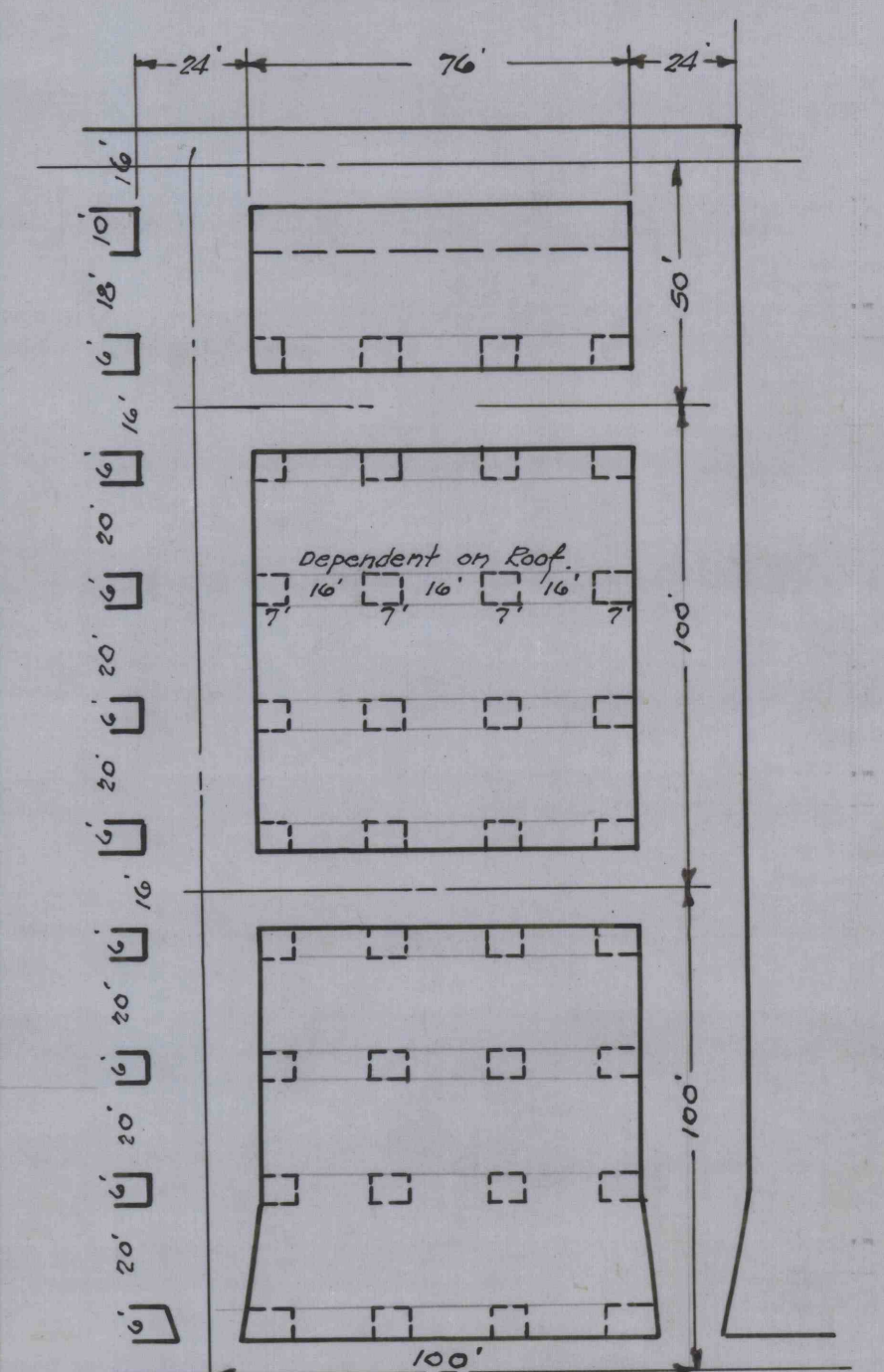
DETAIL OF ROOM PILLARING 1" = 40'
