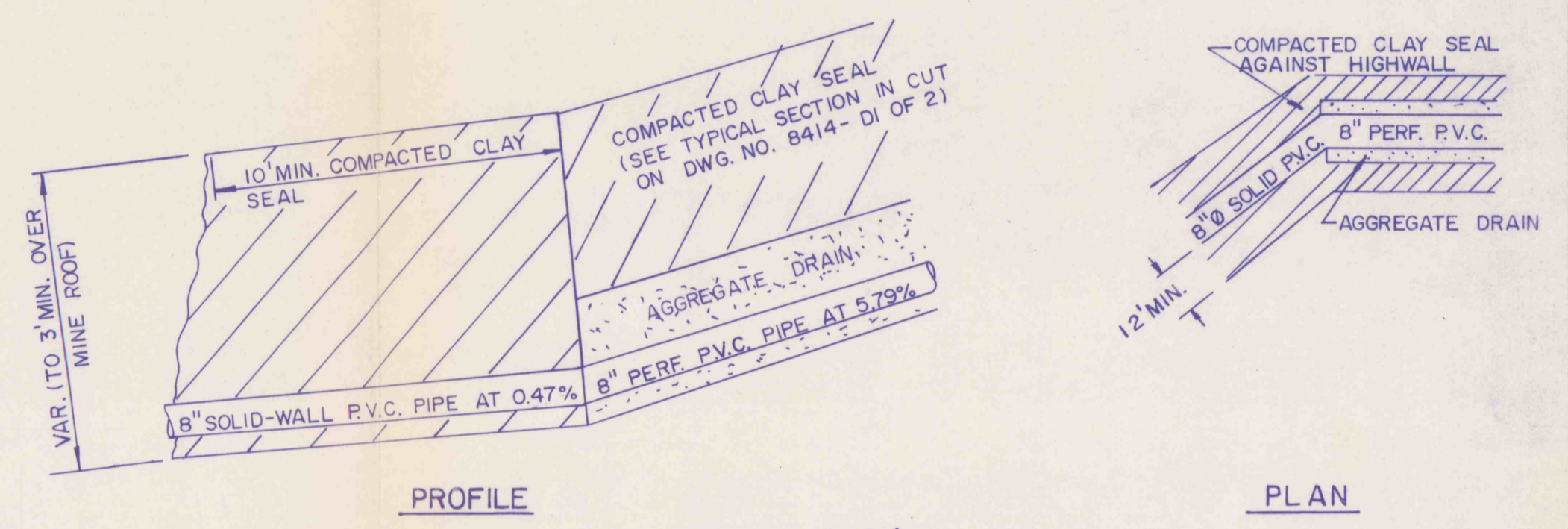
DETAIL "B" No Scale
