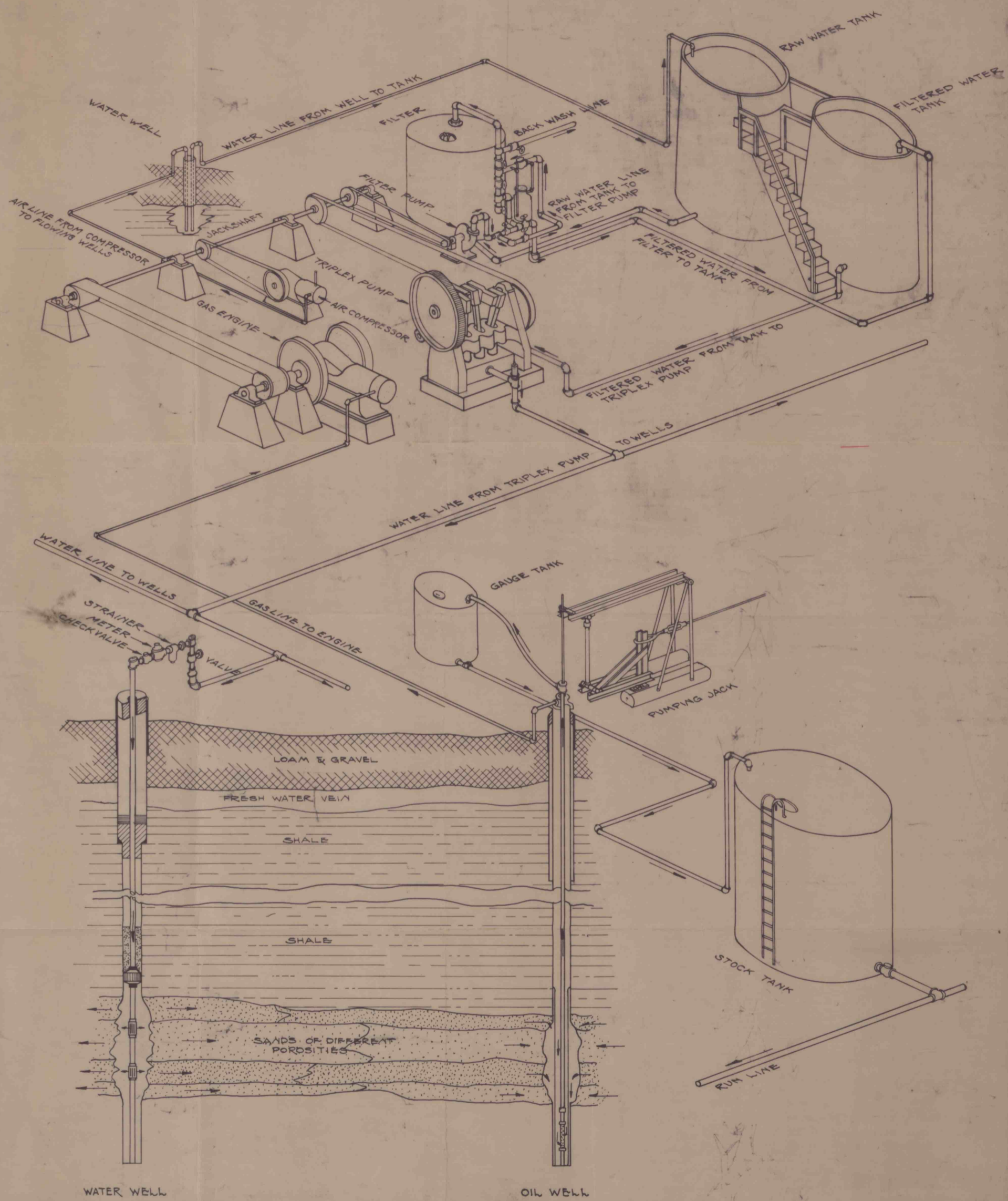
THE SLOAN AND ZOOK COMPANY BRADFORD PA. METHOD OF OIL RECOVERY BY WATER FLOODING PROCESS IN THE BRADFORD FIELD MVB:eam May 12 1930.
