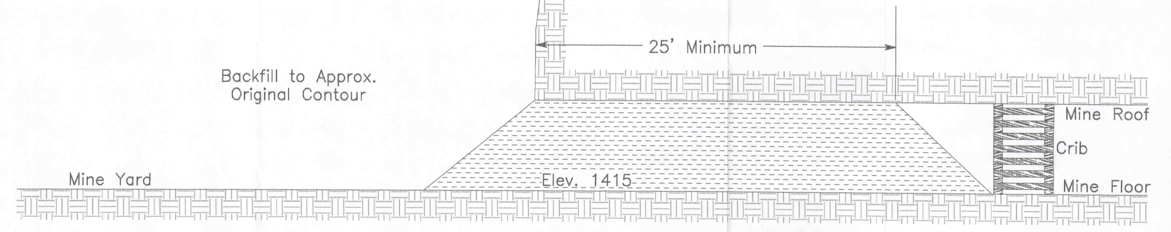
Mine Seal - Side View
