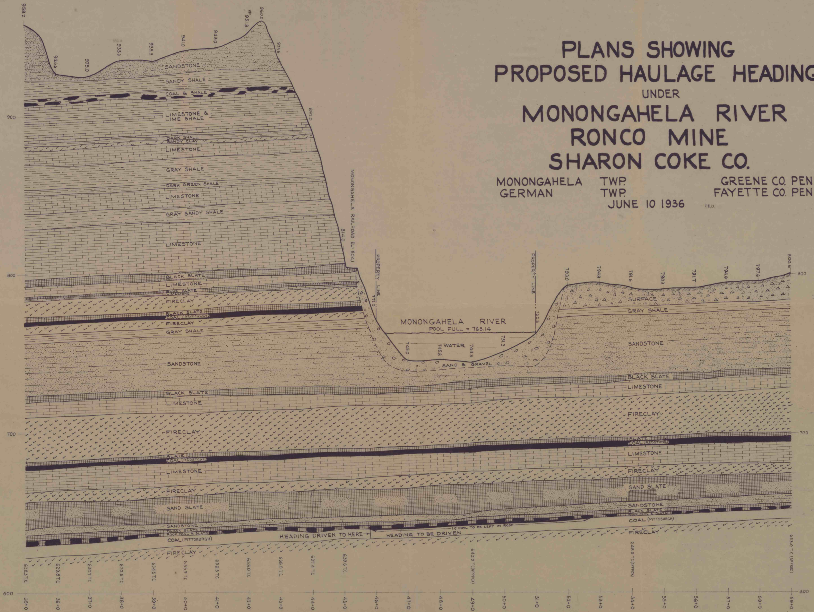
STRATA ABOVE PROPOSED HEADINGS SCALE HOR. 1" = 100' VER. 1" = 20'
