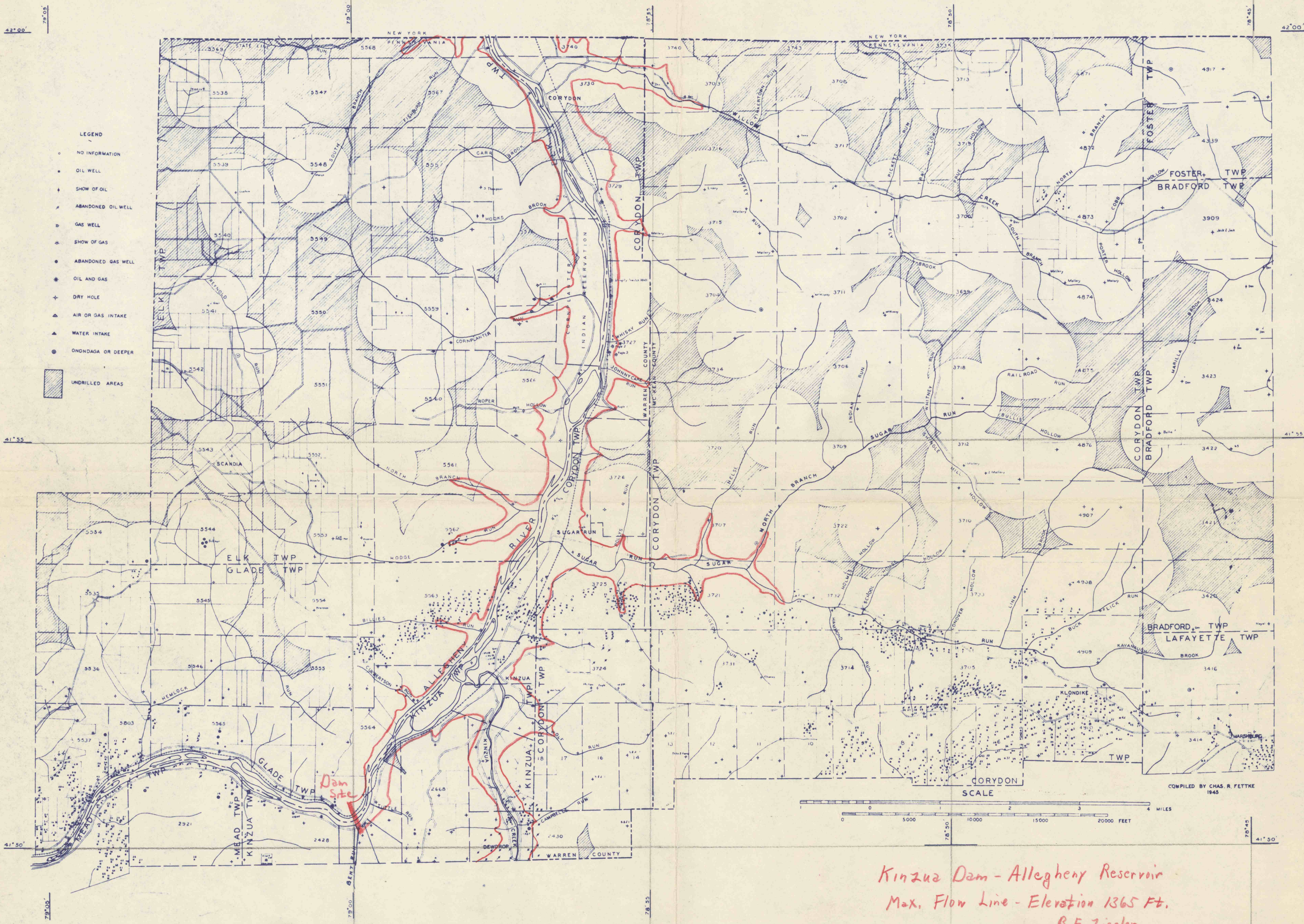
UNDRILLED AREAS OF THE NORTHERN PART OF THE KINZUA QUADRANGLE
