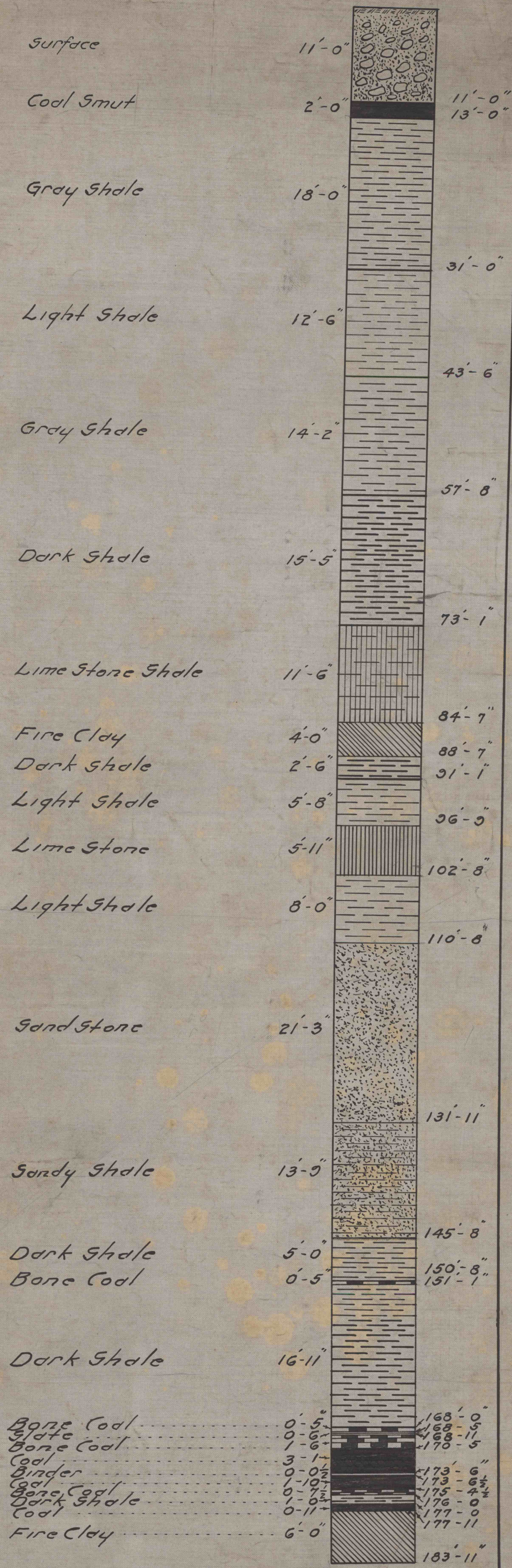
SECTION OF MEASURES IN DIAMOND DRILL HOLE NO. 2 ON THE LATROBE COAL CO'S PROPERTY IN DERRY TWP., WESTMORELAND CO. SCALE: 1"=10' Geo. Silberman & Co. ENGINEERS JUNE 4, 1909.
