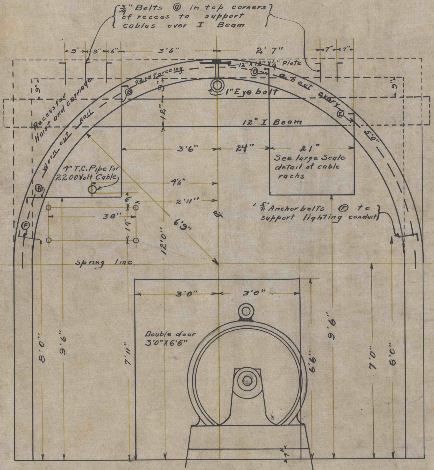
END & SECTION B-B
