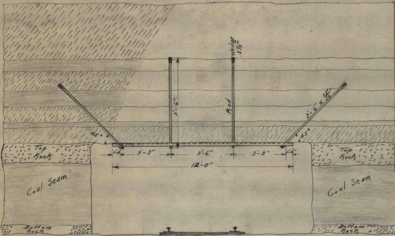
Cross Section of Mine Entry Showing Channel Suspension Supports
