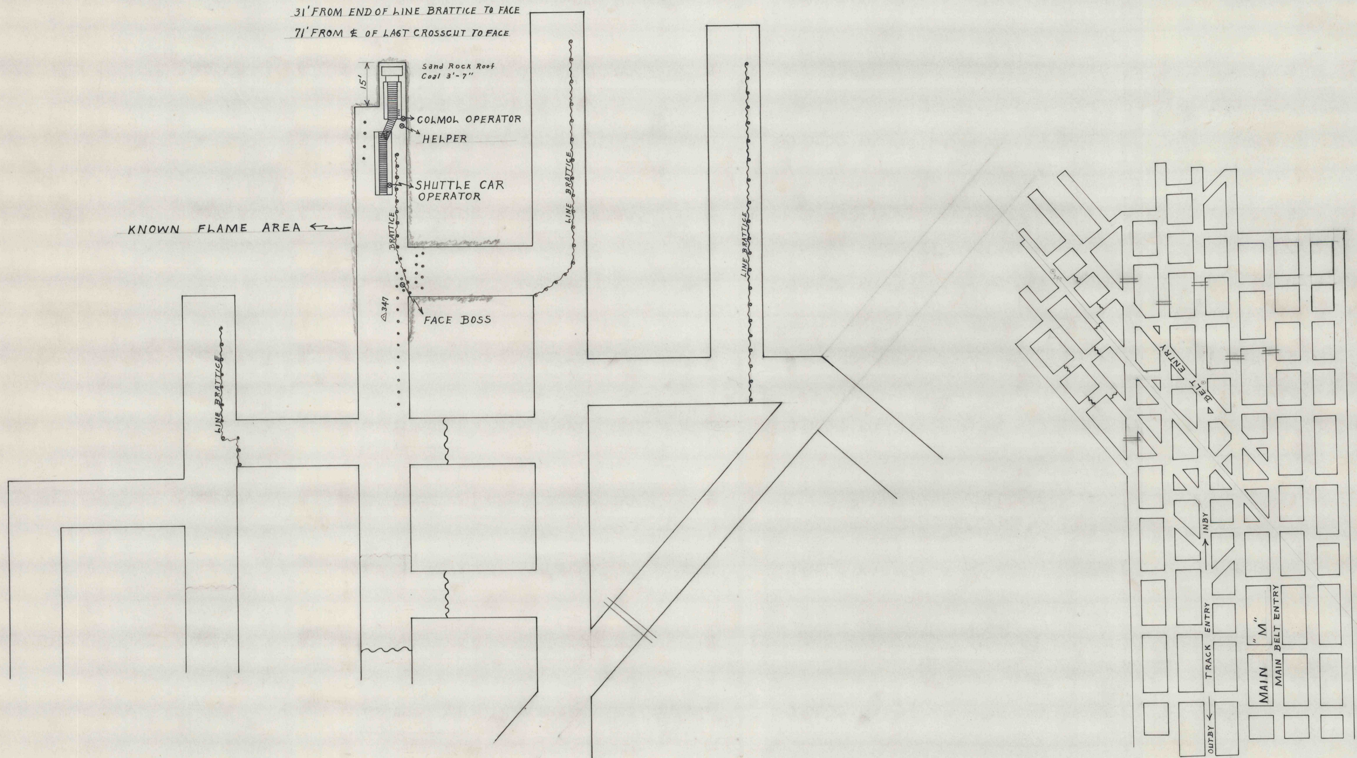
LANCASHIRE No 15 MINE MAIN "M" SECTION IGNITION AREA MAIN ENTRY OCTOBER 26 1961 SECOND SHIFT SCALE 1"=20'
