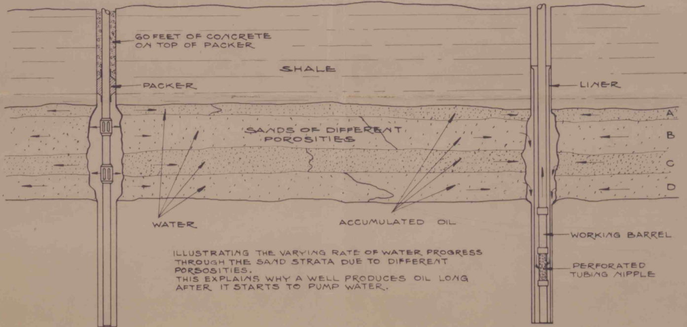
OIL WELL
