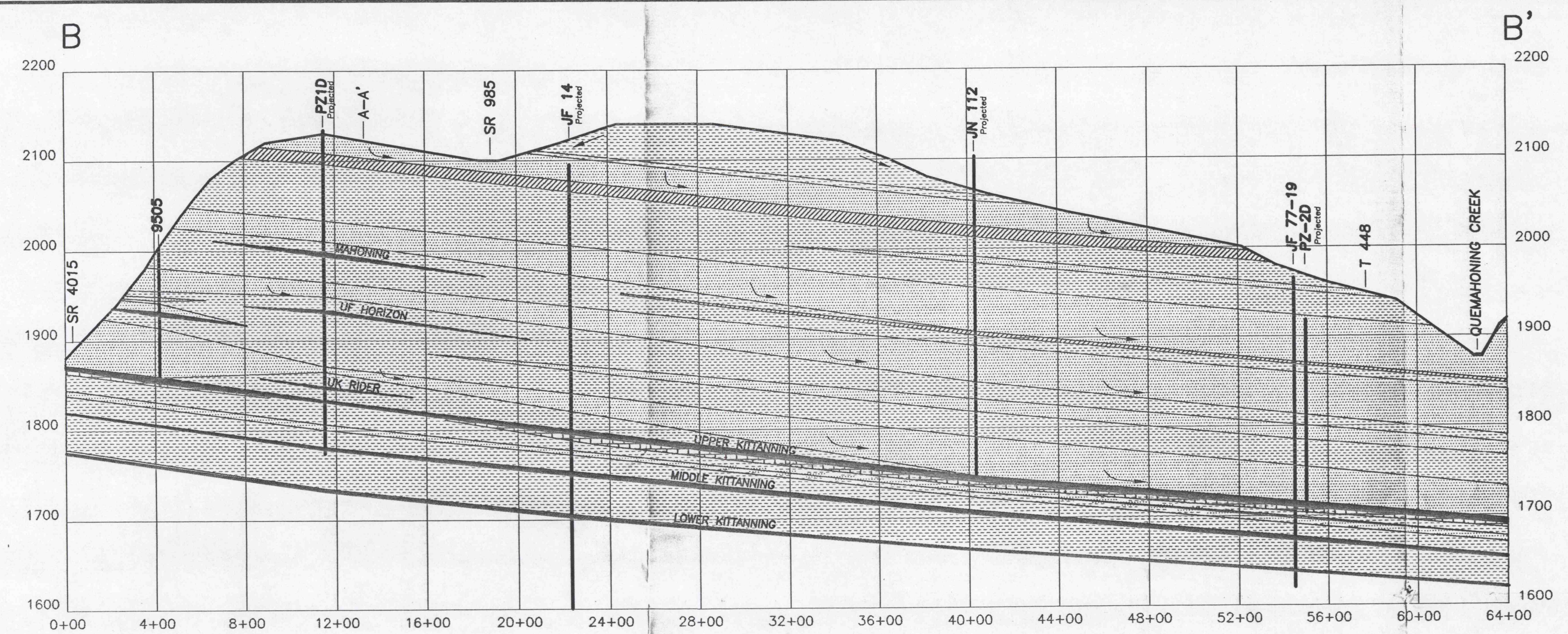
CROSS SECTION B - B' HORIZONTAL SCALE: 1" = 400' VERTICAL SCALE: 1" = 100' VERTICAL EXAGGERATION = 4x
