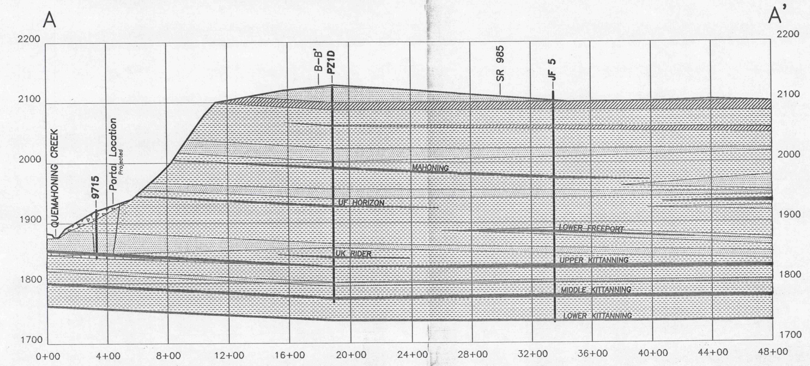
CROSS SECTION A - A' HORIZONTAL SCALE: 1" = 400' VERTICAL SCALE: 1" = 100' VERTICAL EXAGGERATION = 4x GROUND WATER FLOW IS BASICALLY PERPENDICULAR TO SECTION A-A' AND TOWARD THE VIEWER
