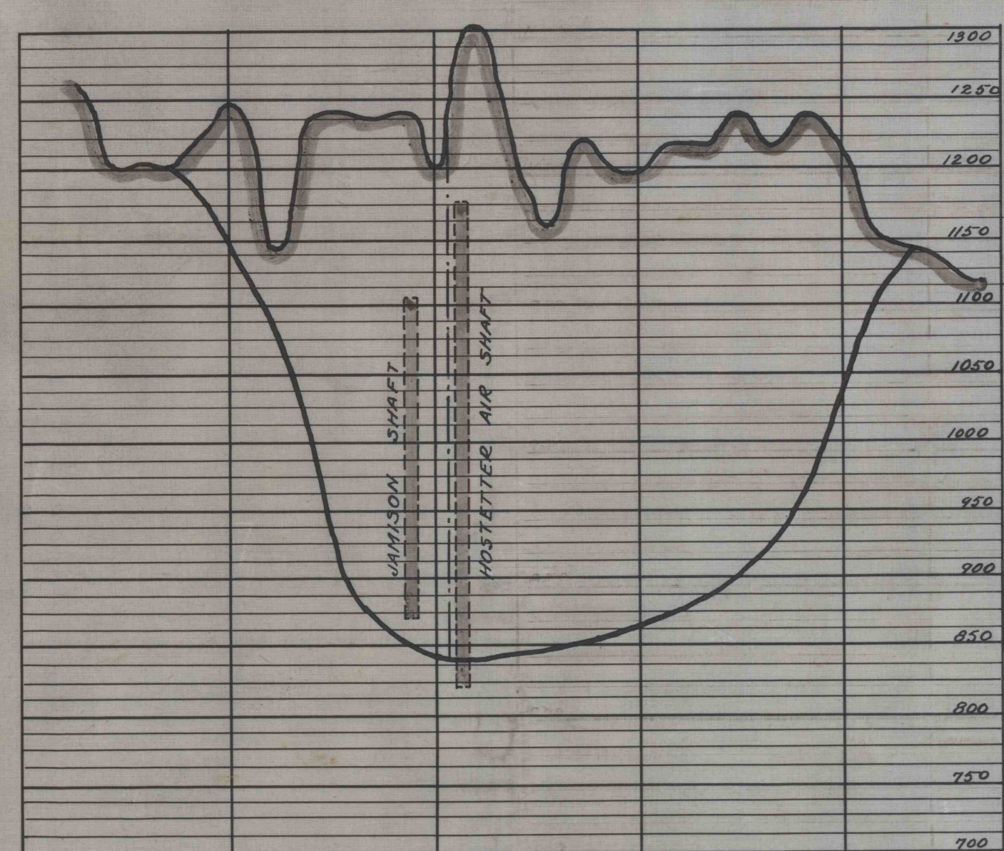
SECTION F-F
