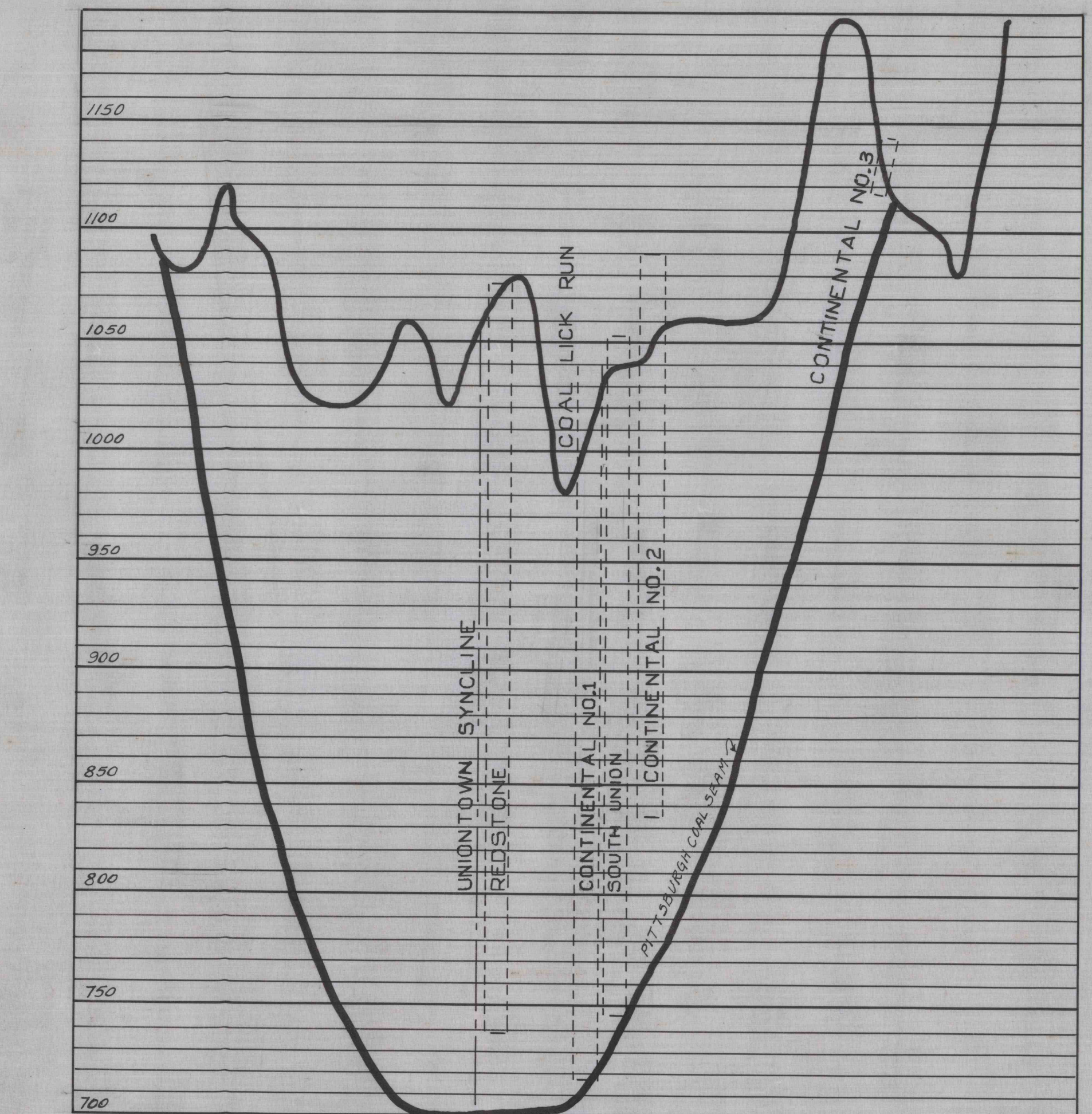
Section '2-2'
