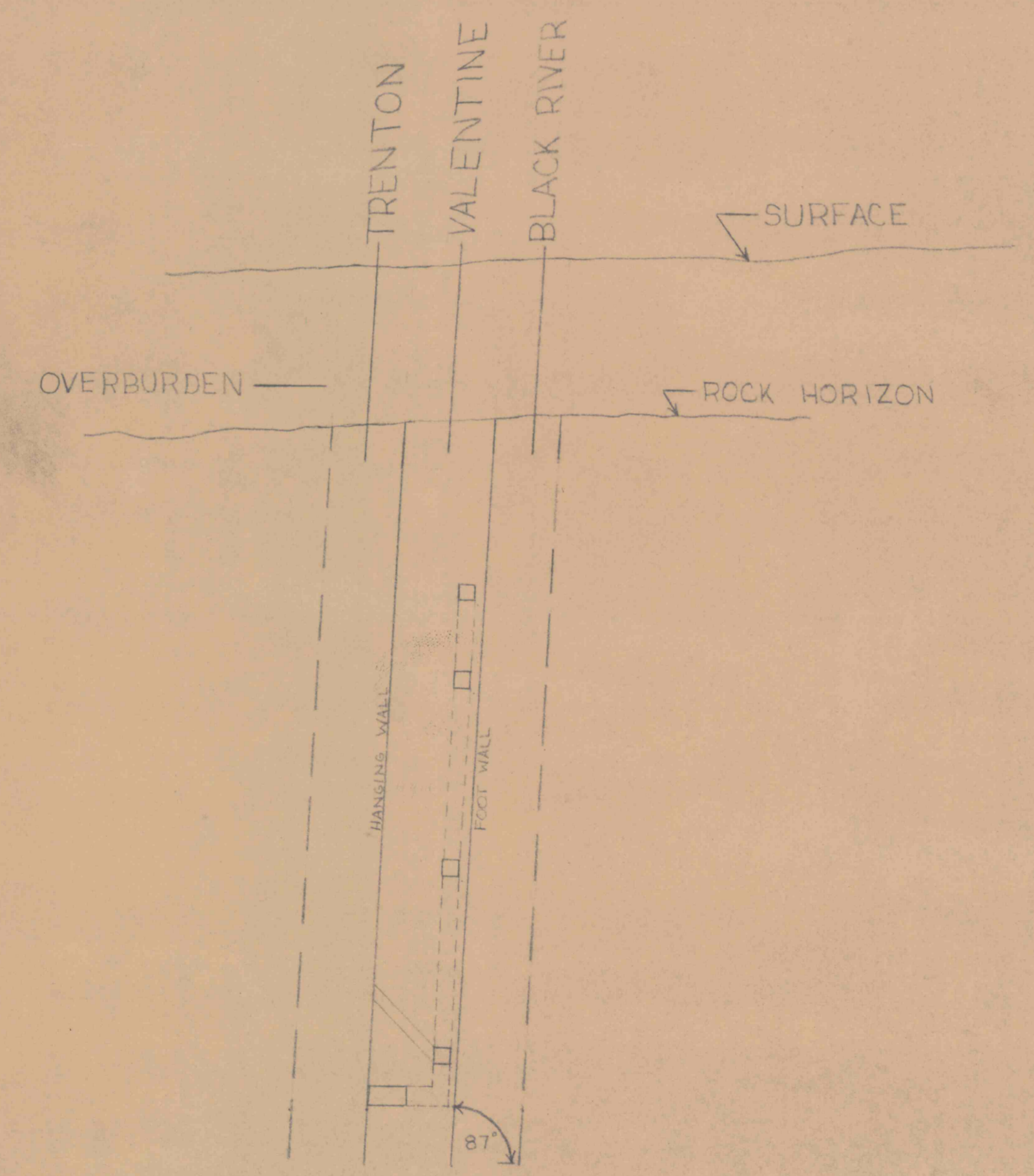
TYPICAL CROSS-SECTION
