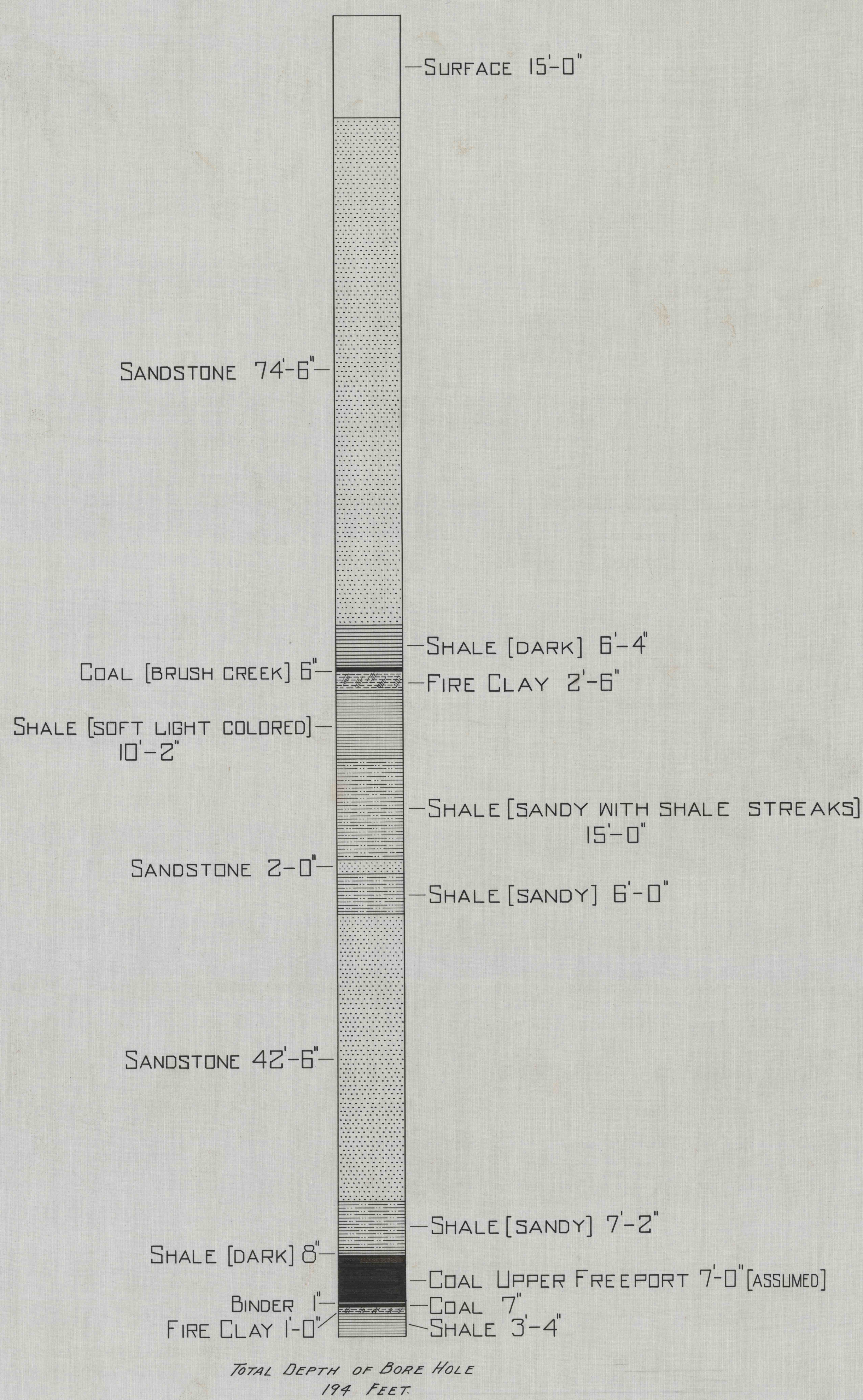
STRATA SHOWN BY DIAMOND DRILL HOLE HUBBARD SHAFT SCALE 1 INCH = 10 FEET
