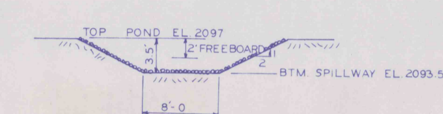
SPILLWAY SECTION SCALE 1"=10'
