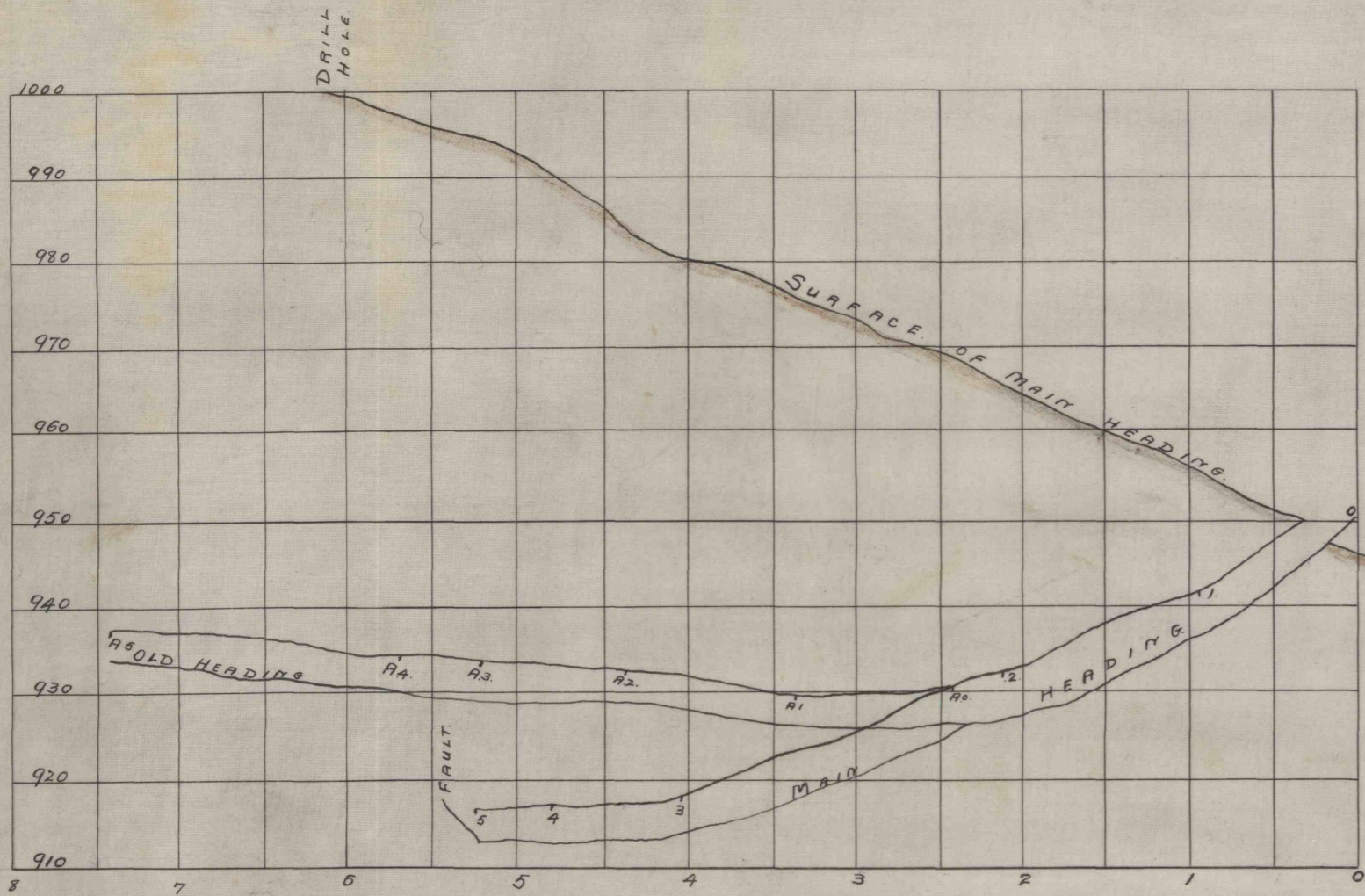
PROFILE SCALE { Vertical 1" = 20' Horizontal 1" = 100'
