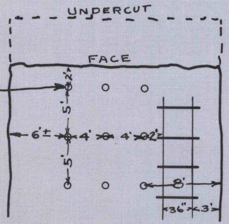
TYPICAL TIMBERING AT WORKING FACE
