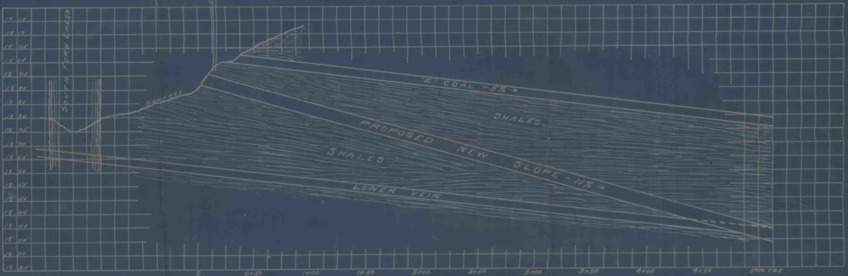
SECTION ON LINE OF NEW SLOPE vertical - 25' = 1" SCALE Horizontal - 50' = 1"
