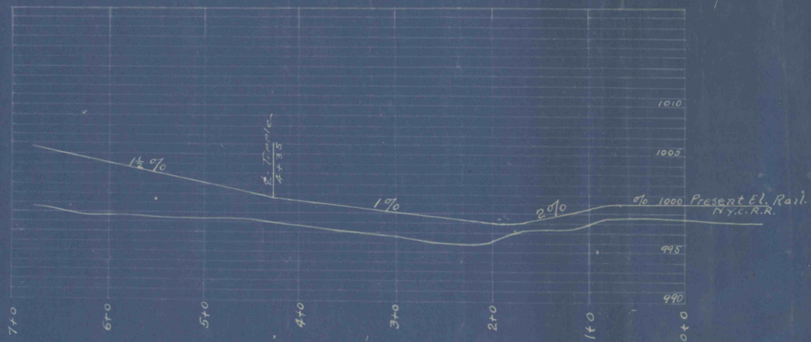
PROFILE - TOP OF RAIL Scales { Hor 1" = 100' Vert 1" = 10'
