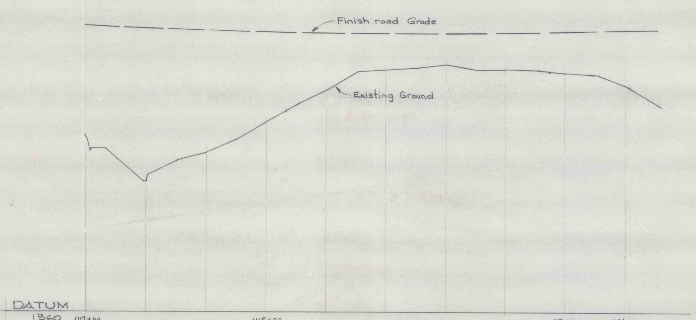
PROFILE W.B.
