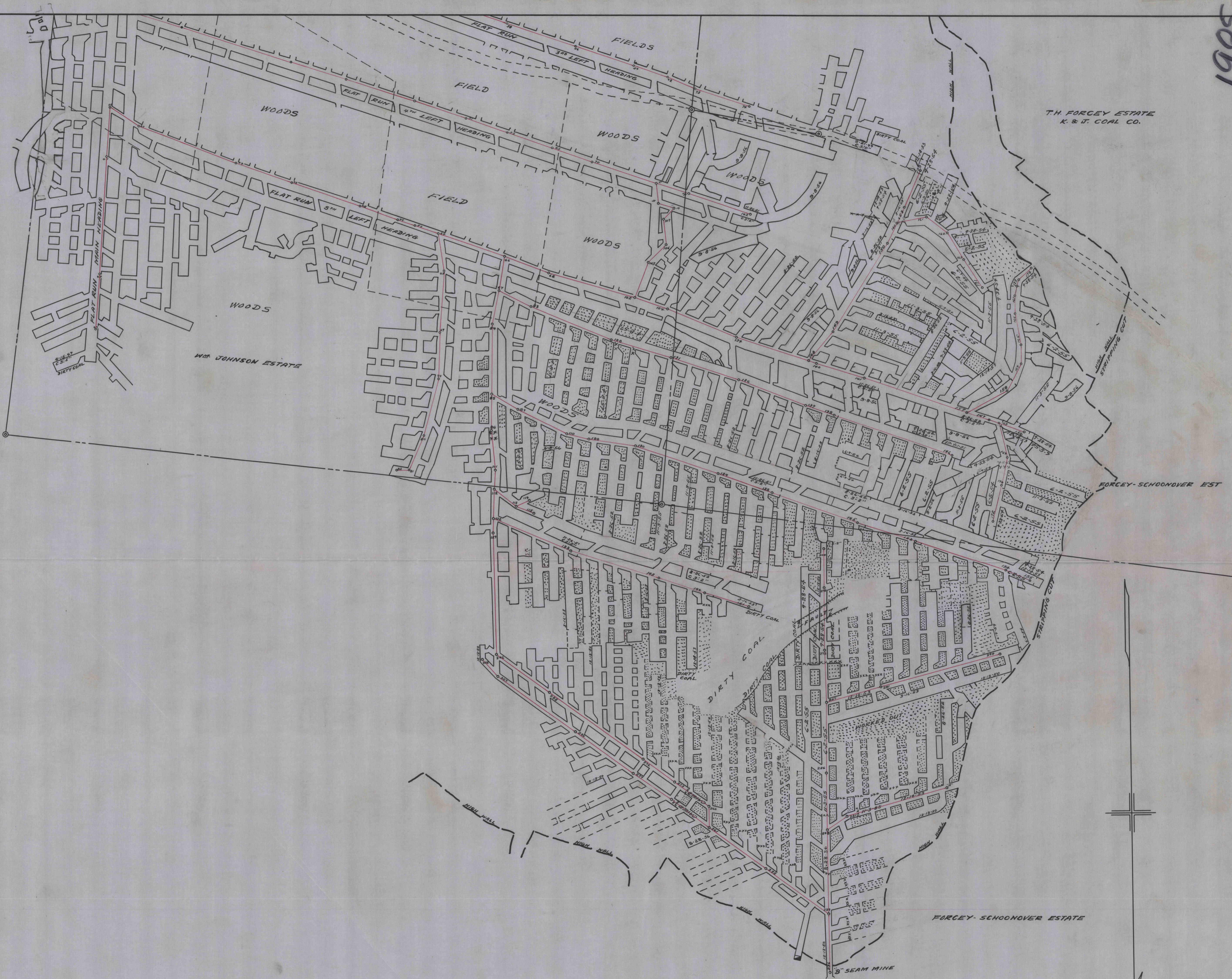
— MAP OF GREEN VALLEY & FLAT RUN MINES — — OPERATED BY KRISTIANSON & JOHNSON COAL CO. — — GRAHAM TOWNSHIP CLEARFIELD COUNTY, PENNA. — — SCALE 1"=100' — (C.D. 354) — DEC. 22, 1950 — — BERNARD LUGAS ENGR. —
