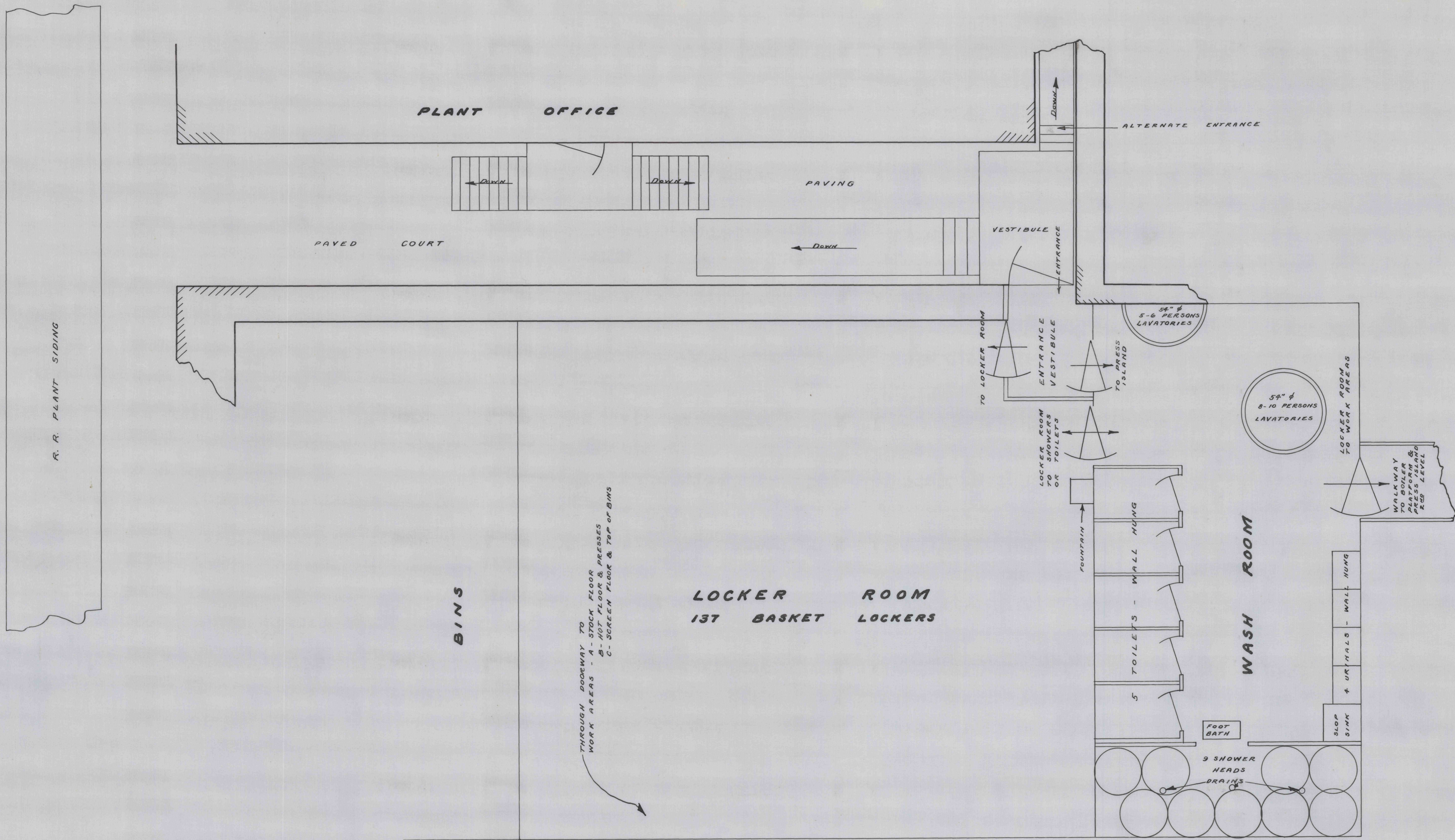
NORTH AMERICAN REFRACTORIES CO. CLEVELAND, OHIO PLAN VIEW OF PROPOSED WASH ROOM AND LOCKER ROOM AT CURWENSVILLE PLANT SCALE: 3/8" = 1 FT. DRAWN - J.R.H., JR. DRAWN FROM P.B. & I. PRINT E-8-65, SHEET No. E1 No. C.L. FREDRICK DRAWING
