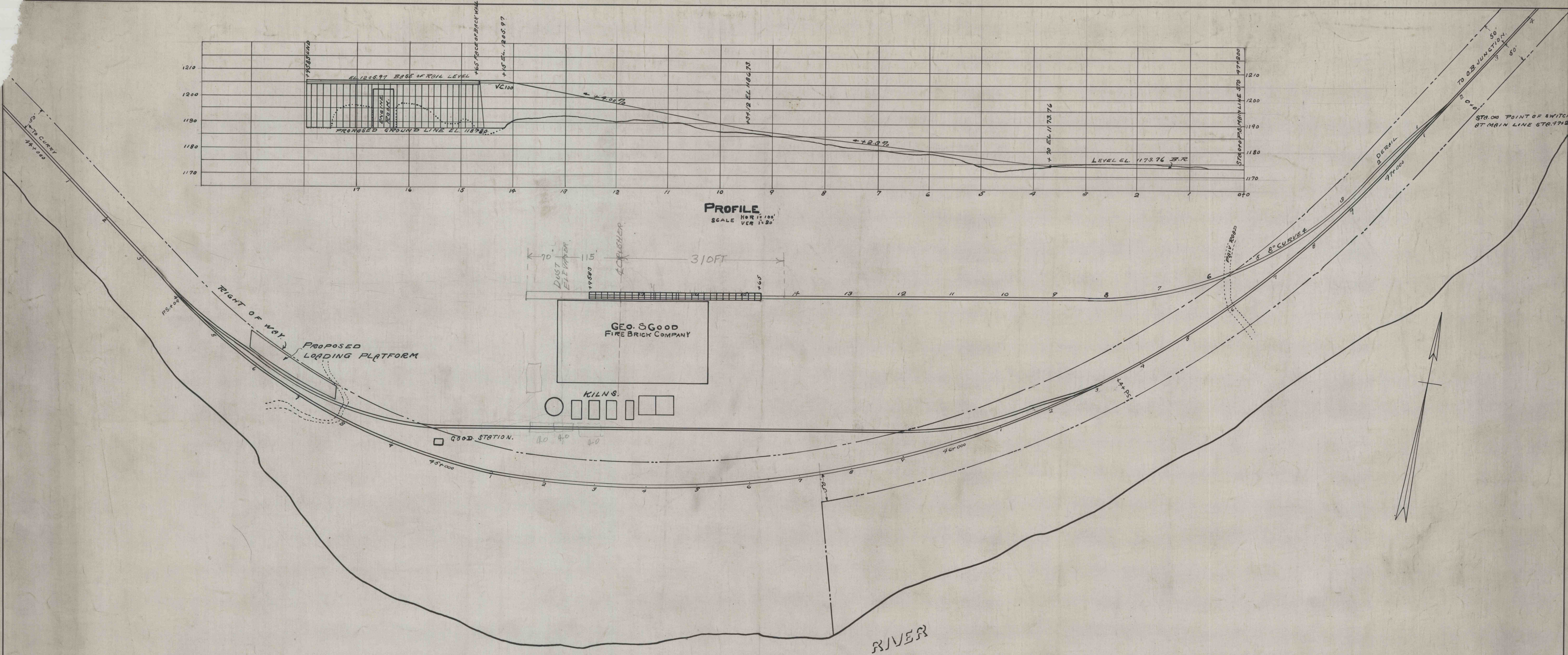
SUSQUEHANNA LOCATION PLAN SCALE 1" = 100'
