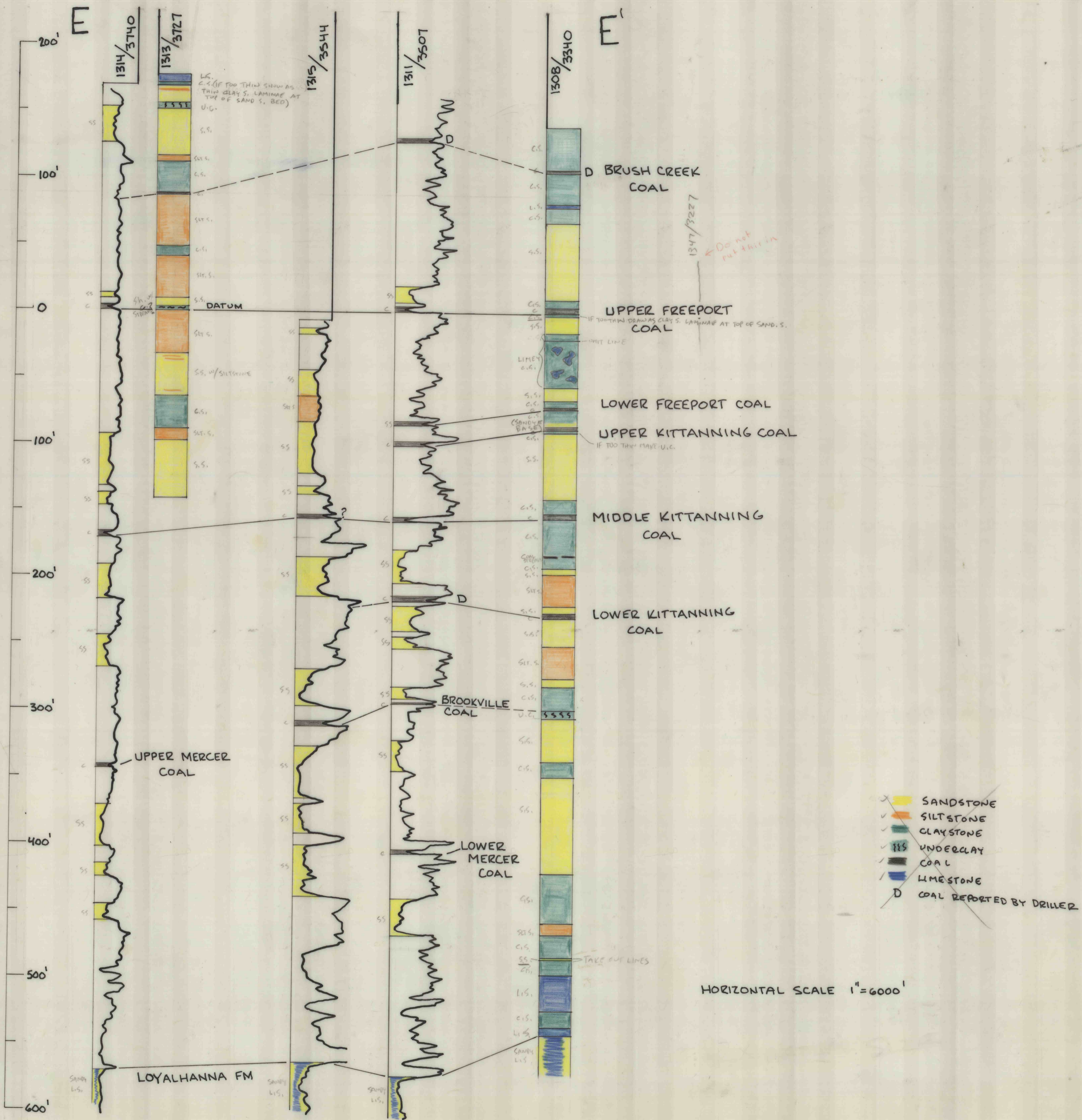
FIG 32- GAS WELL CORRELATION DIAGRAMS
