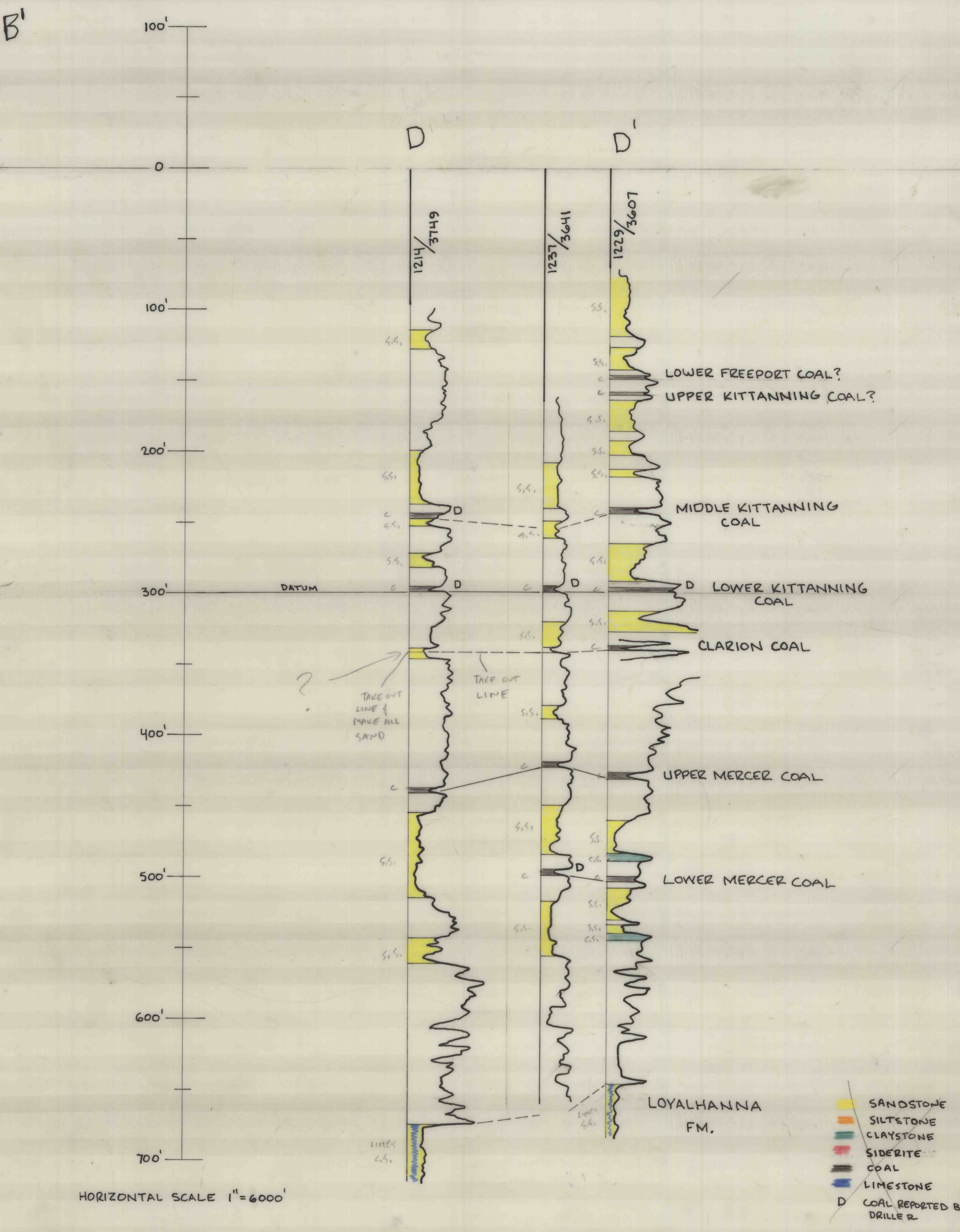
FIG 31.- GAS WELL CORRELATION DIAGRAMS
