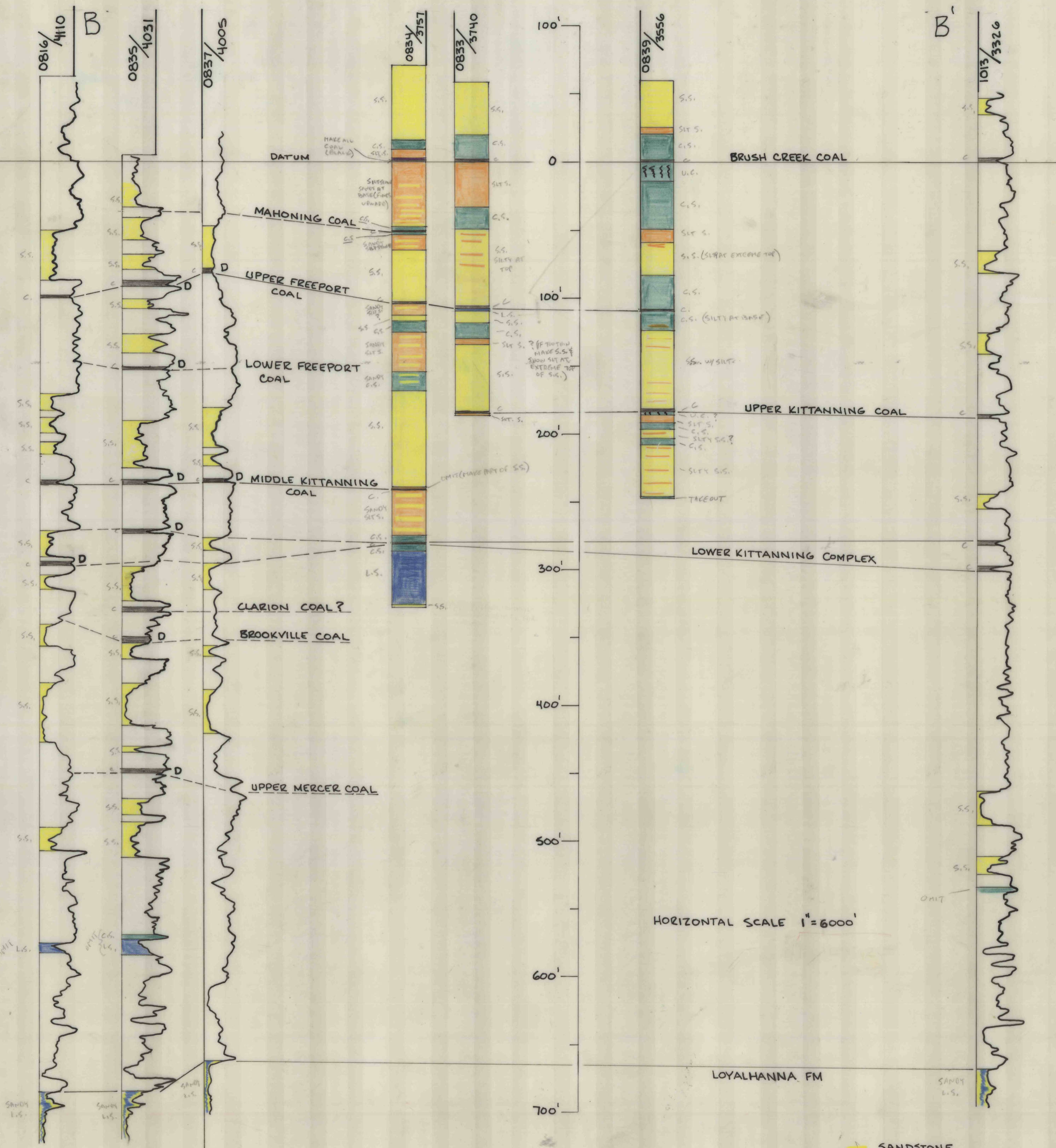
FIG. 30 - GAS WELL CORRELATION DIAGRAMS
