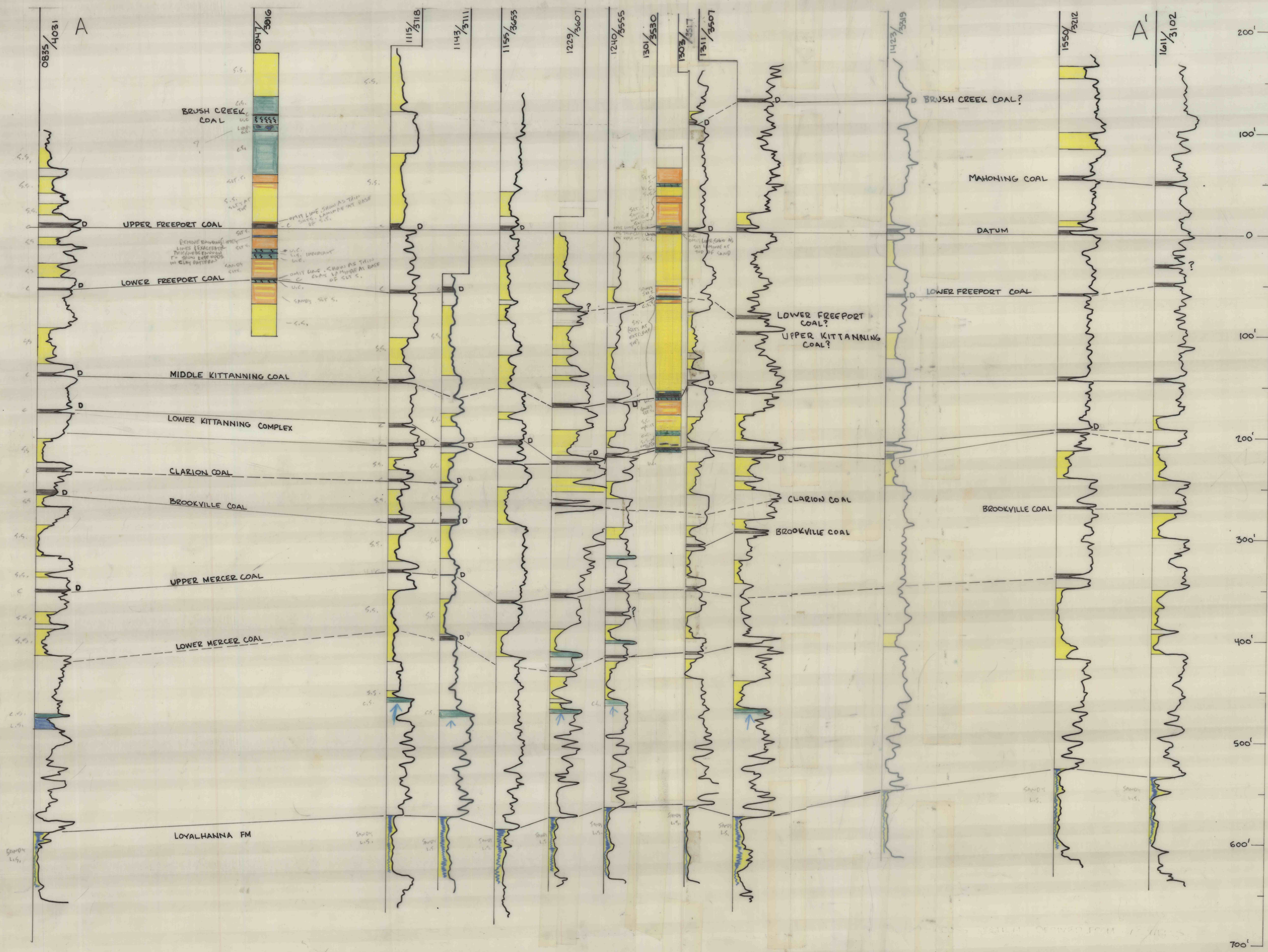
FIG. 29 - GAS WELL CORRELATION DIAGRAMS
