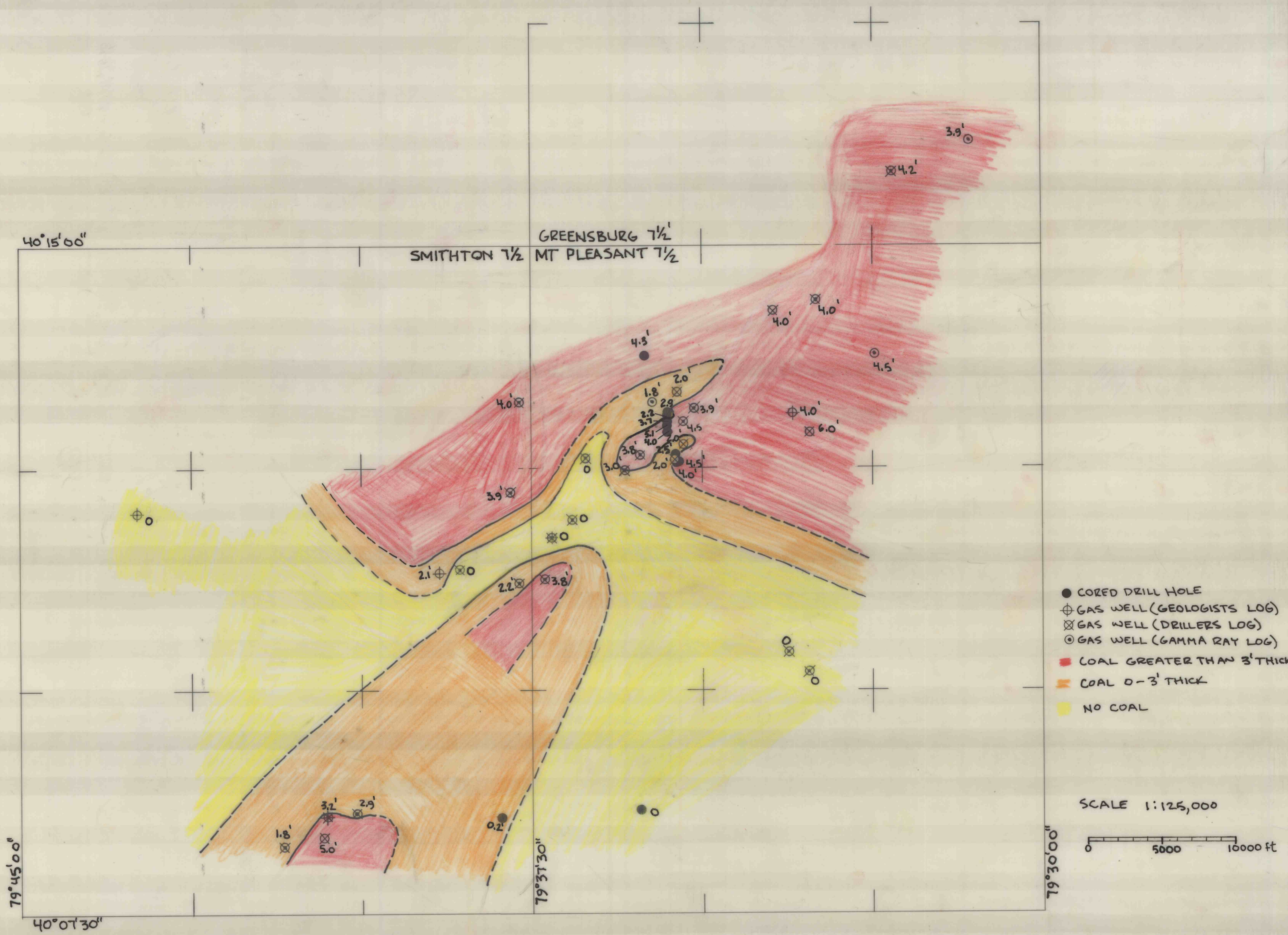
FIG 33 - DISTRIBUTION & THICKNESS MAP OF MIDDLE KITTANNING COAL
