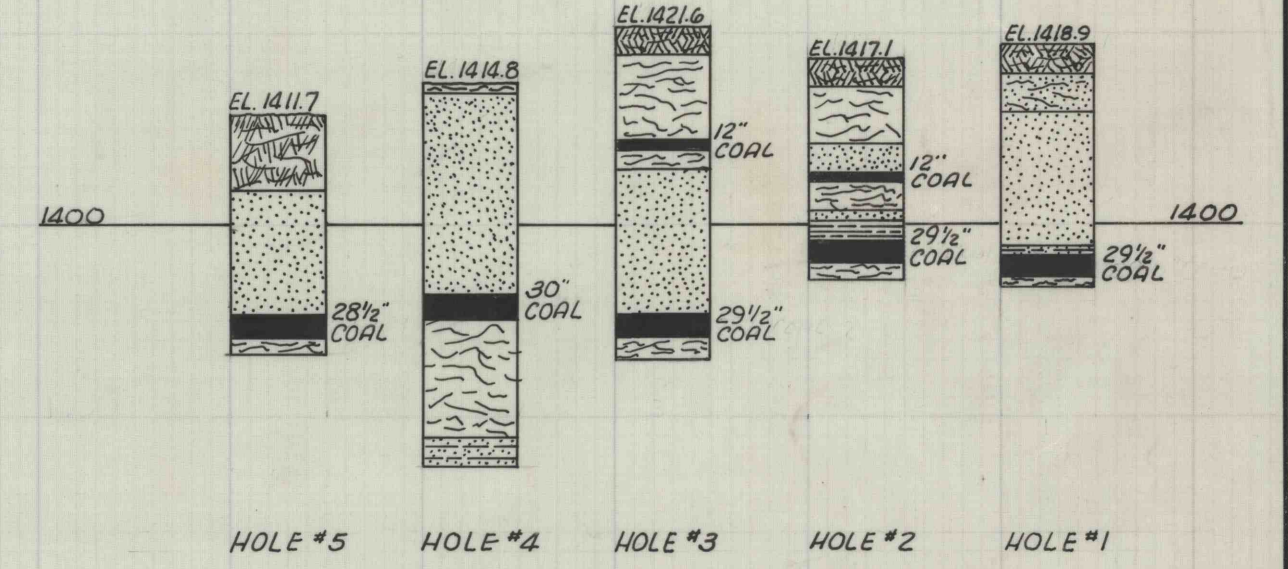
COLUMNAR SECTIONS SCALE: 1" = 20'
