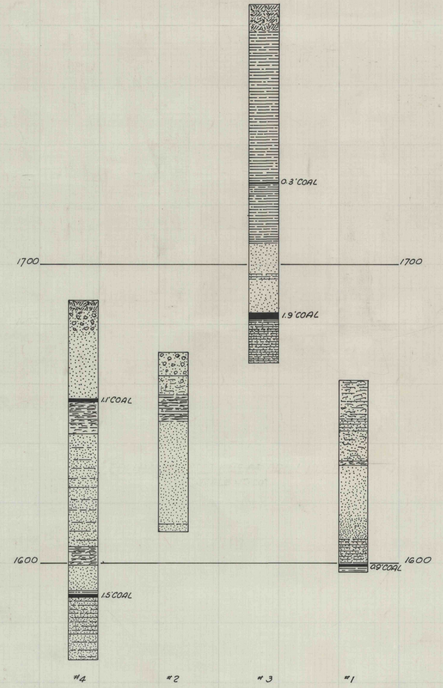
COLUMNAR SECTIONS OF DRILL HOLES SCALE: 1" = 20'
