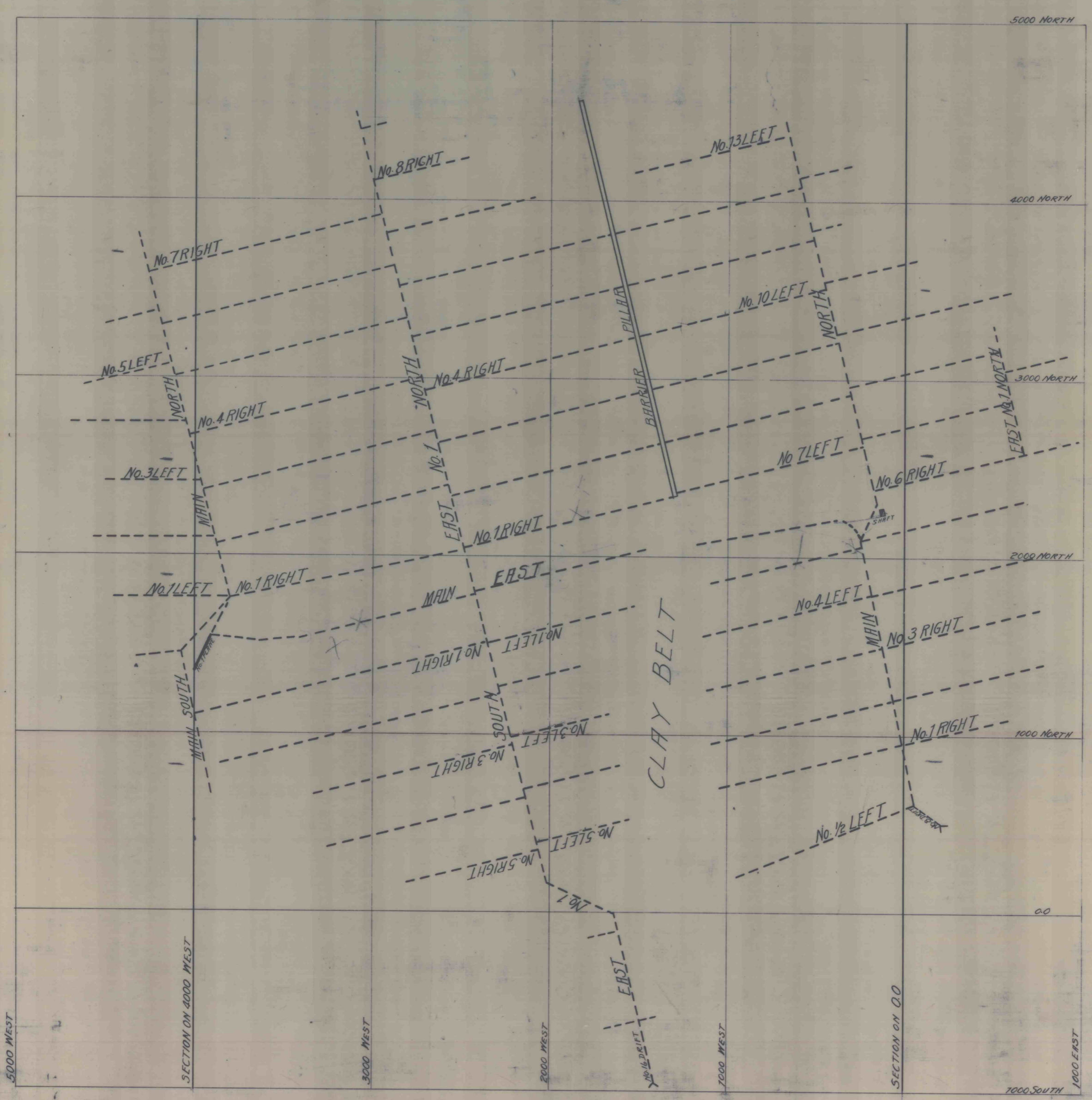
MORGAN VEIN WORKINGS MORRIS RUN PA. SCALE 1"=500' MAY 1923
