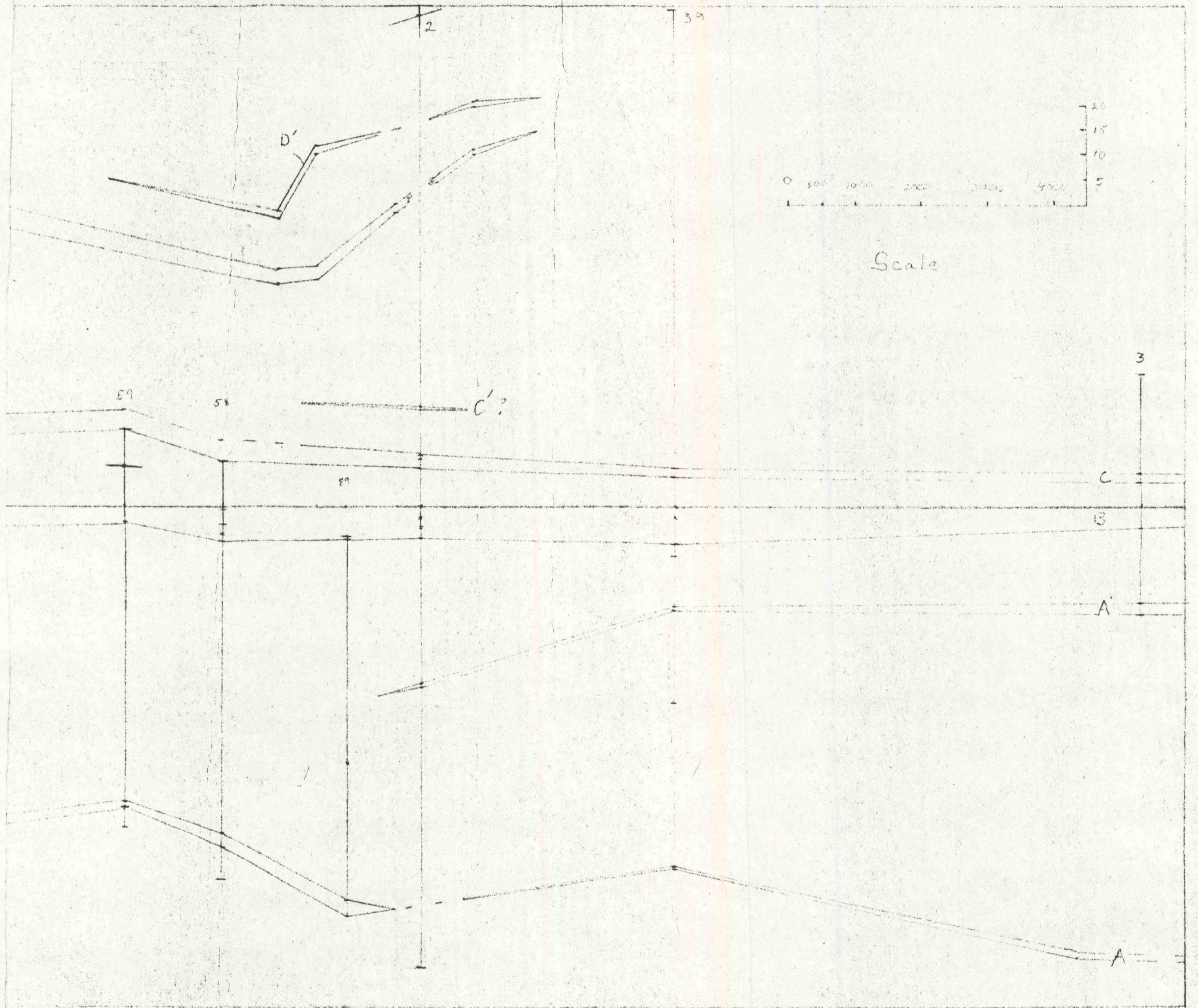
BASIN. (SEE PLATE I FOR DRILL HOLE LOCATIONS)
