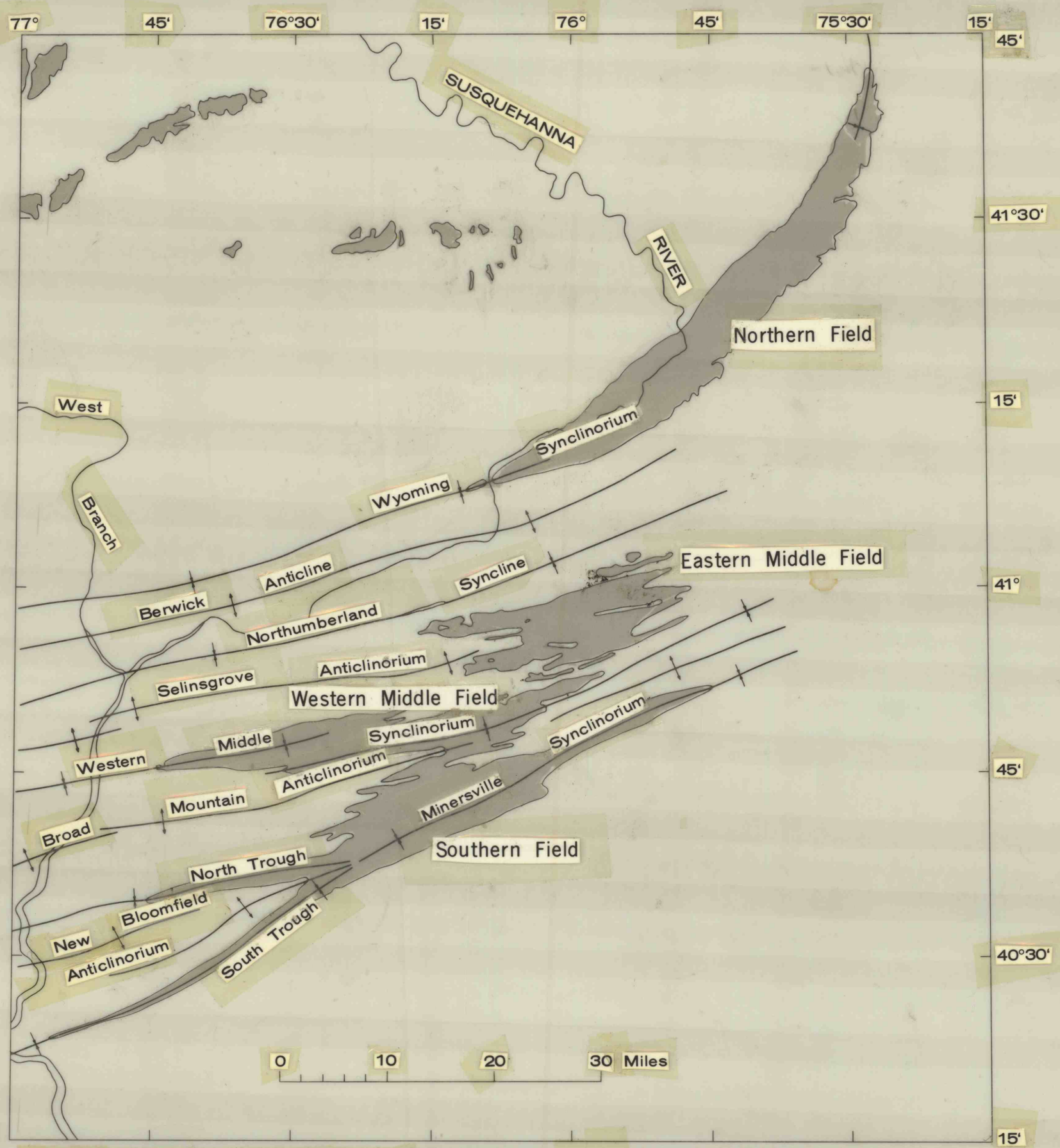
FIGURE 3.--Map showing location of the Anthracite fields in relation to principal structural features.
