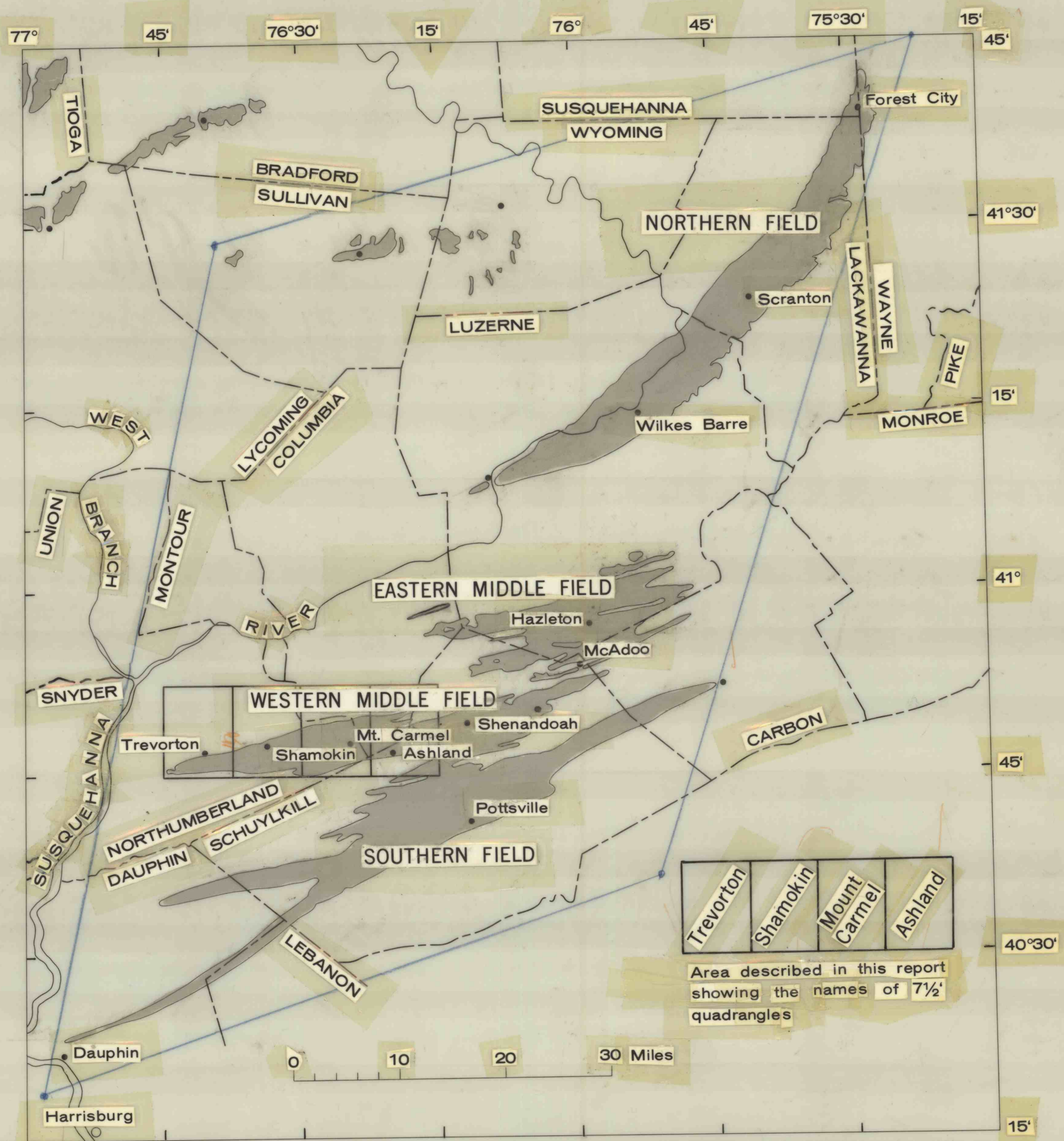
FIGURE 2.--Index map of the Pennsylvania Anthracite region showing location of the Anthracite fields and the area described in this report
