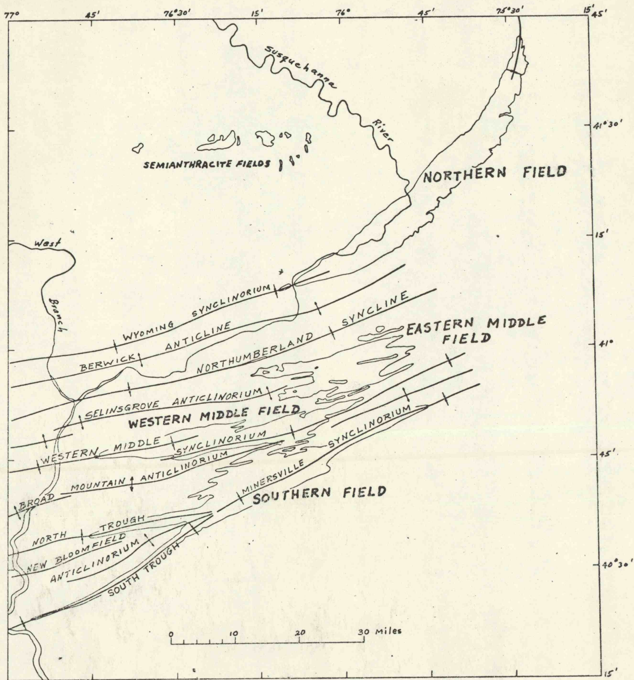
FIGURE 3.--Map showing location of the Anthracite fields in relation to principal structural features.
