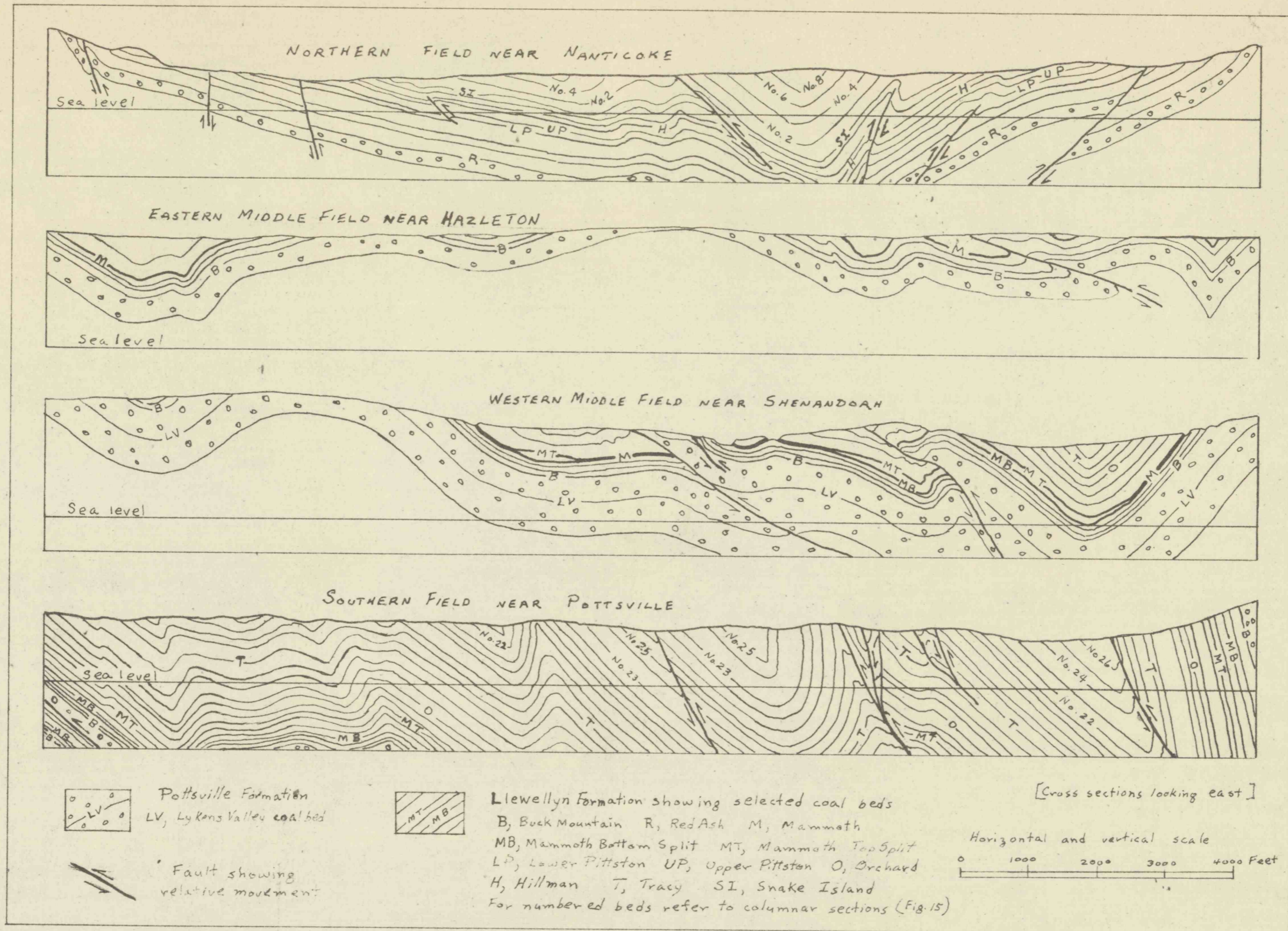
FIGURE 14.— Generalized cross sections of the Pennsylvania anthracite fields
