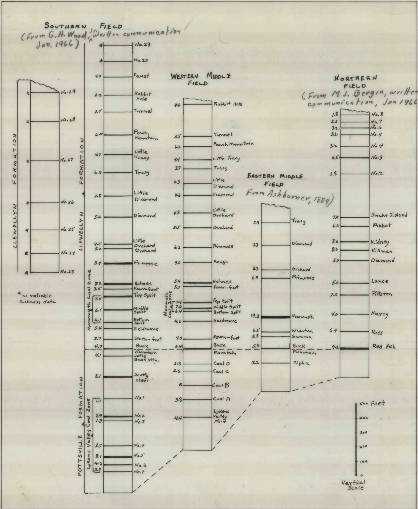
FIGURE 19 - Generalized columnar sections showing names, average thickness of coal, and intervals between coal beds in the Pennsylvania anthracite fields
